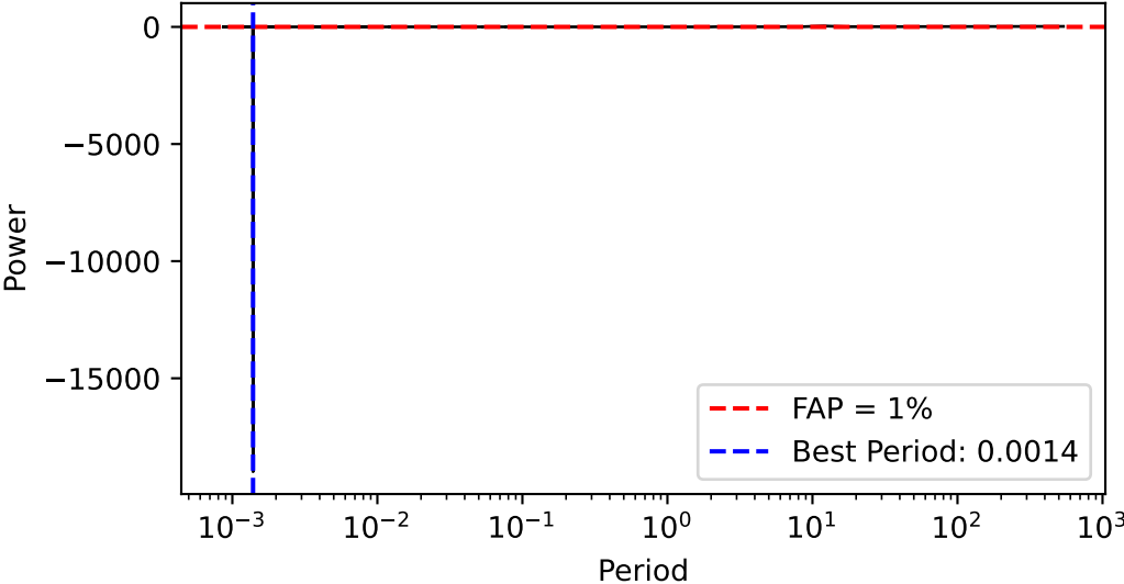
Lomb-Scargle Periodogram
