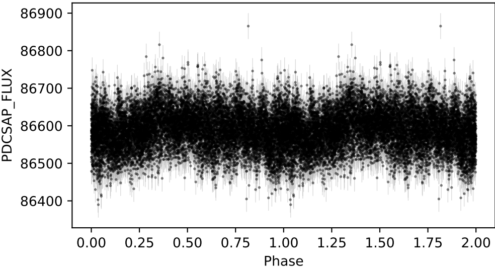
Phase-Folded Light Curve (Period = 0.0014)
