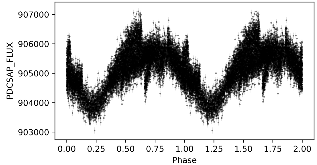
Phase-Folded Light Curve (Period = 0.0014)
