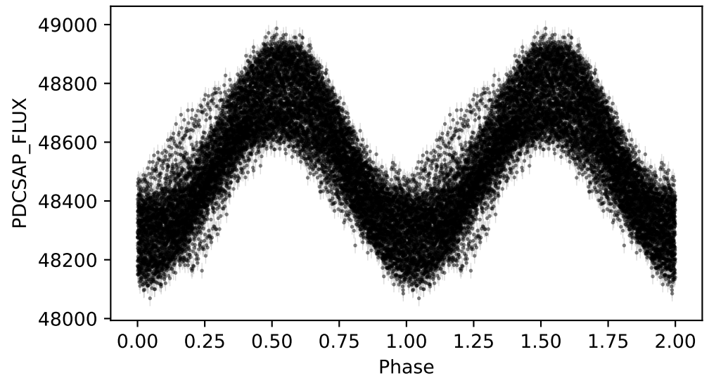
Phase-Folded Light Curve (Period = 0.5960)
