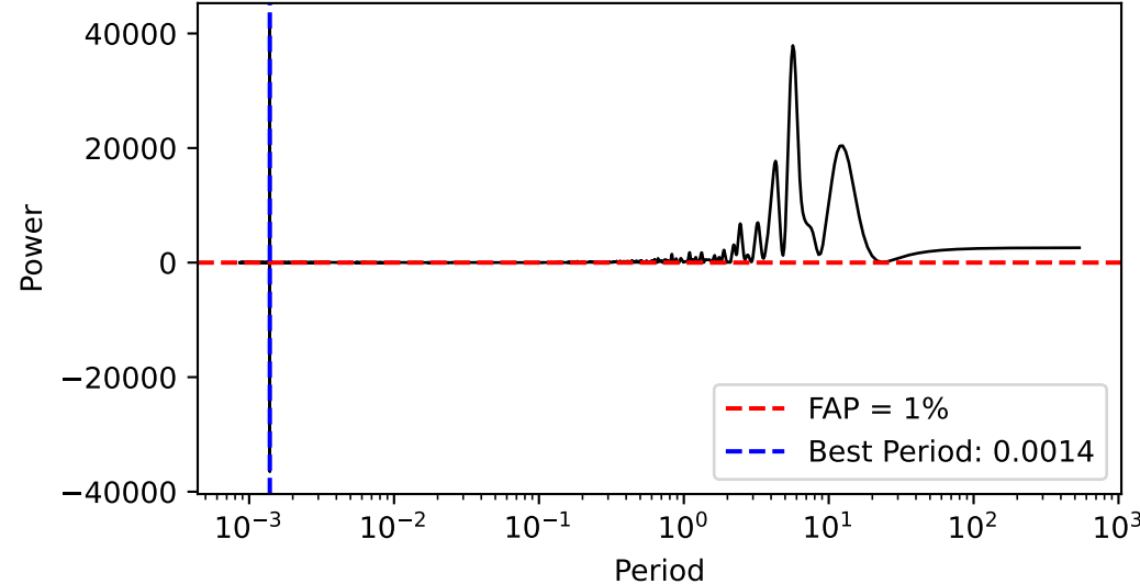
Lomb-Scargle Periodogram
