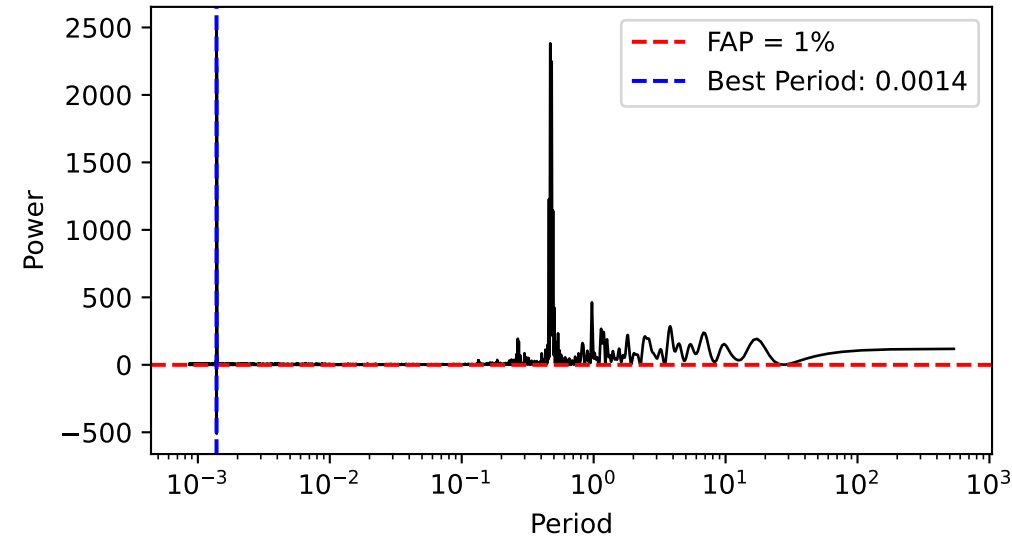
Lomb-Scargle Periodogram
