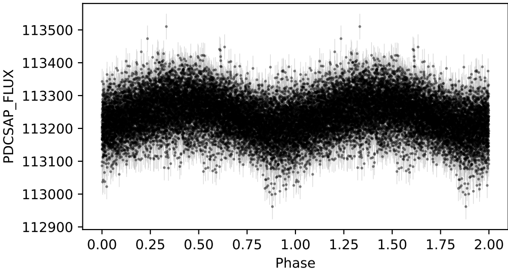
Phase-Folded Light Curve (Period = 0.0014)
