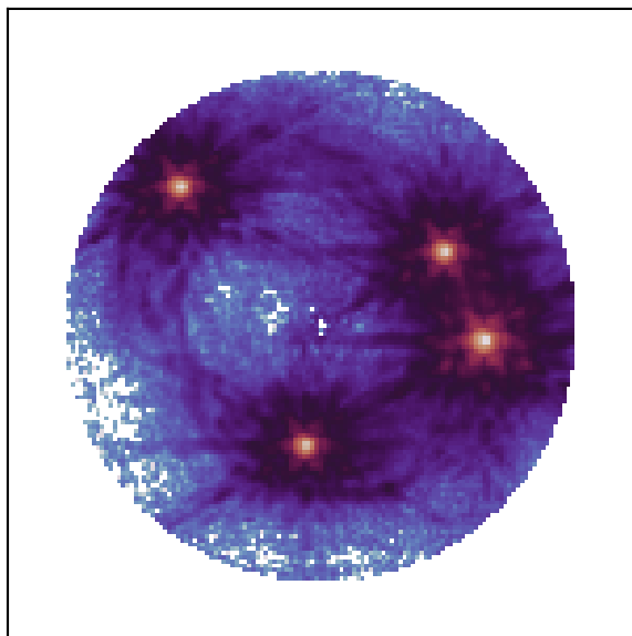
Data (lens light subtracted)
