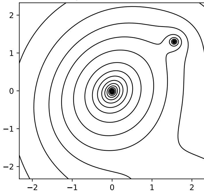
Total convergence (stars + DM + G1/G2)
