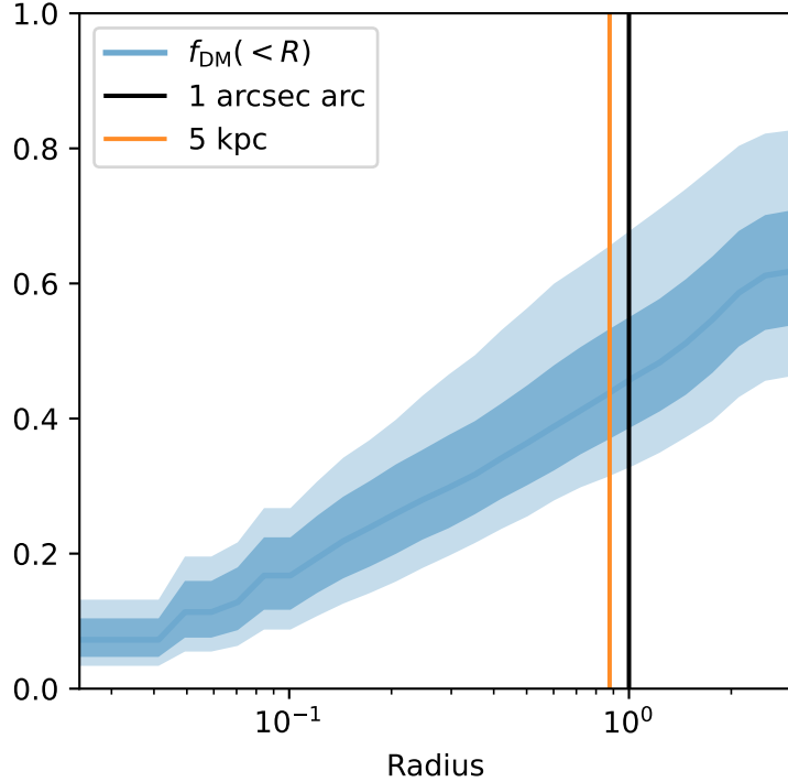
Radial cumulative DM fraction
