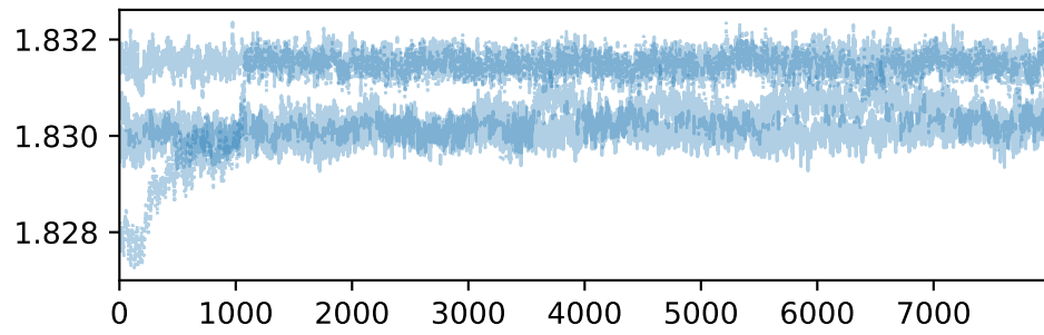
gamma_1
