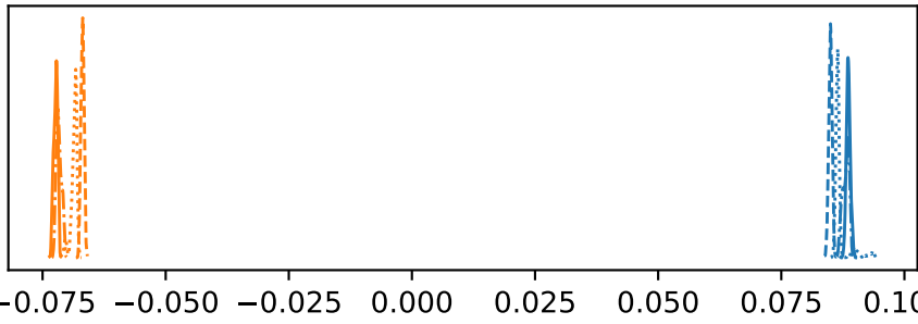
n_source_grid
