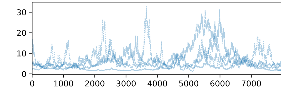
sigma_source_grid
