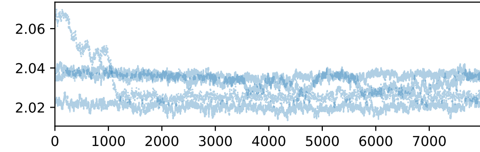
e_1
