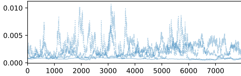
rho_source_grid
