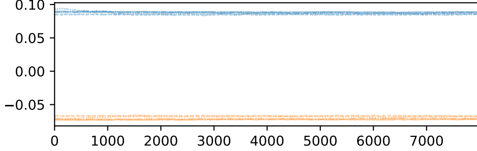
n_source_grid
