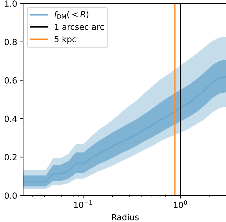
Radial cumulative DM fraction
