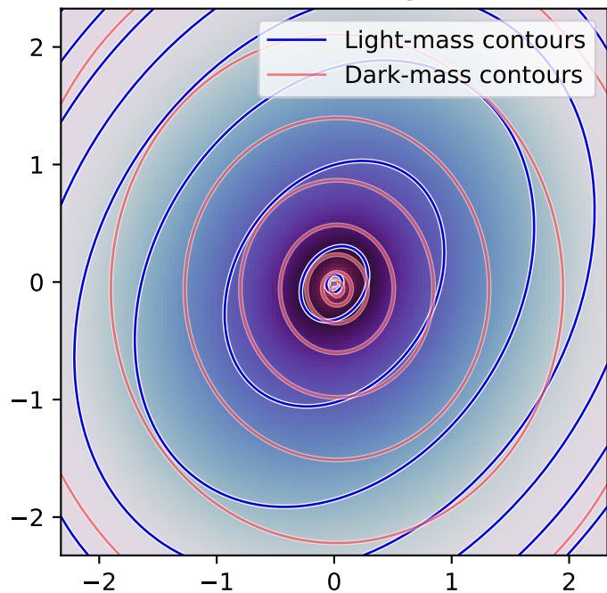
Lens 2D convergence
