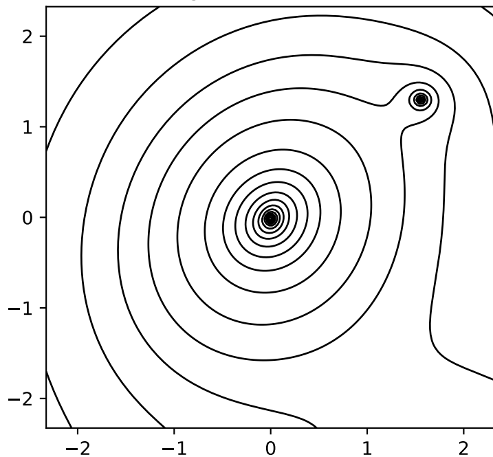
Total convergence (stars + DM + X/G2)
