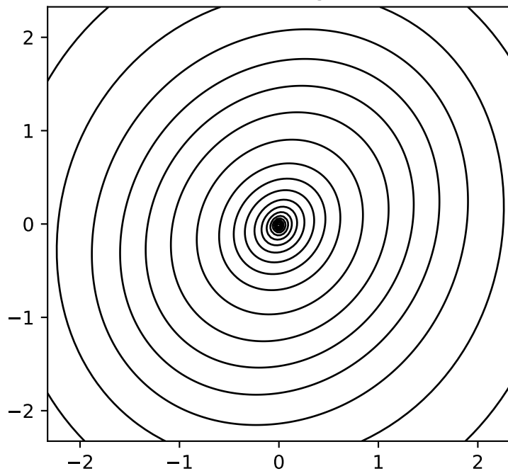
Total convergence
