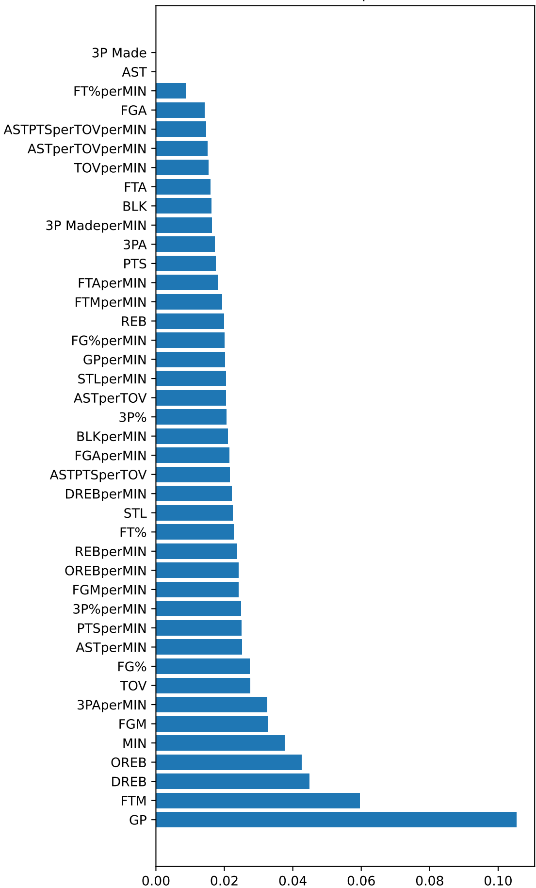
XGBoost Feature Importance (Gain)
