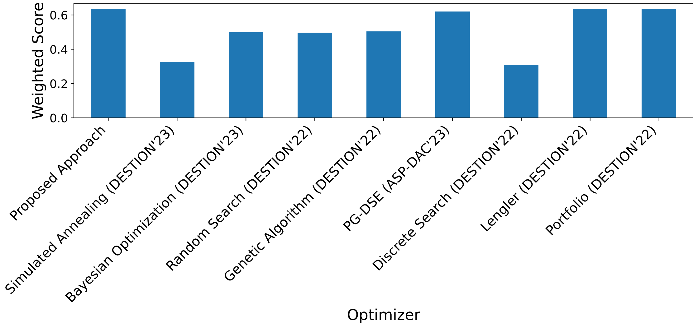
Optimizer Scores
