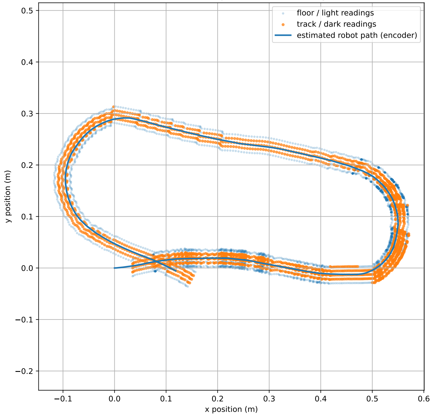
Pololu 2D Route Map from Line Sensor Logs
