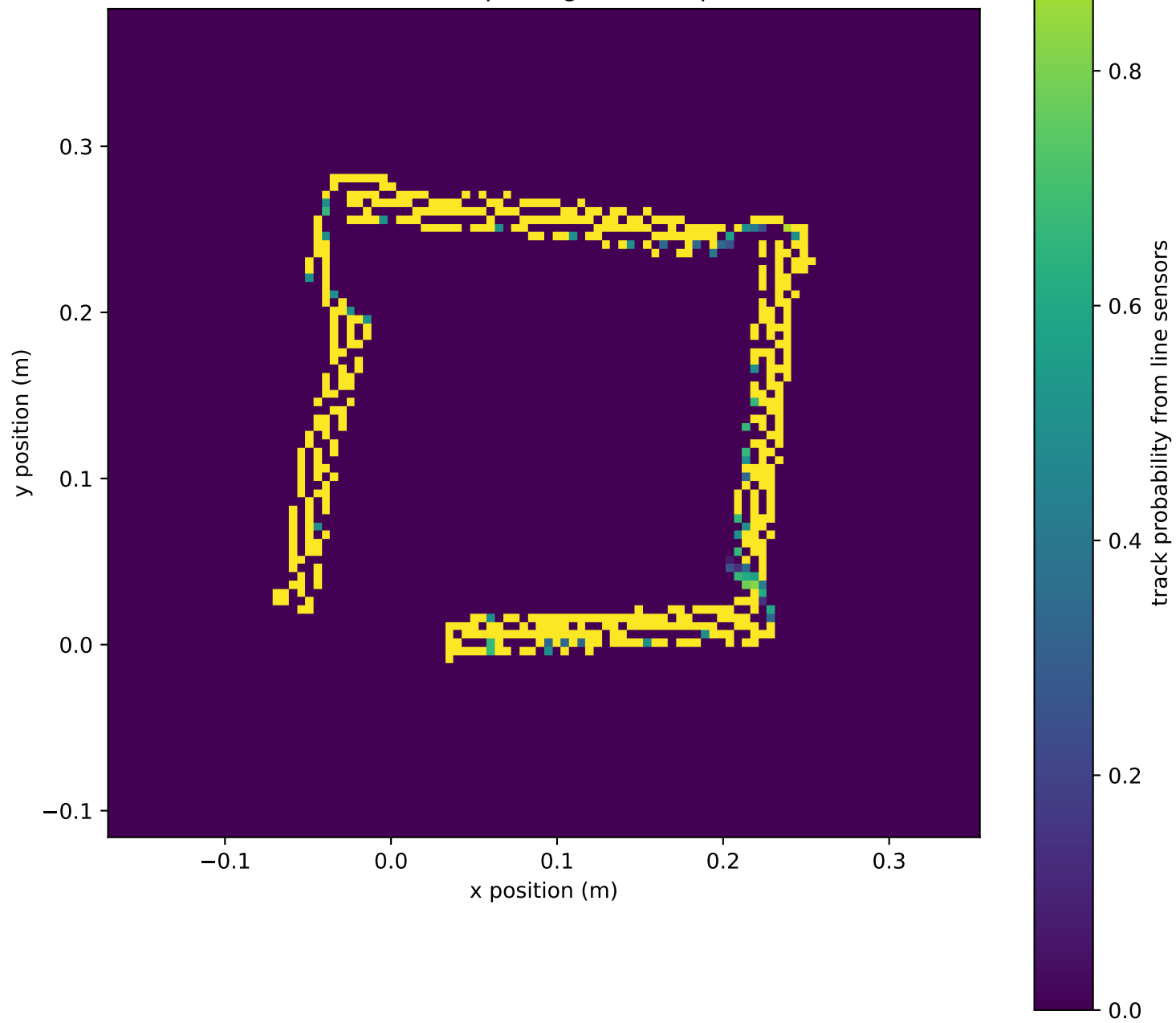
2D Track Map using encoder pose
