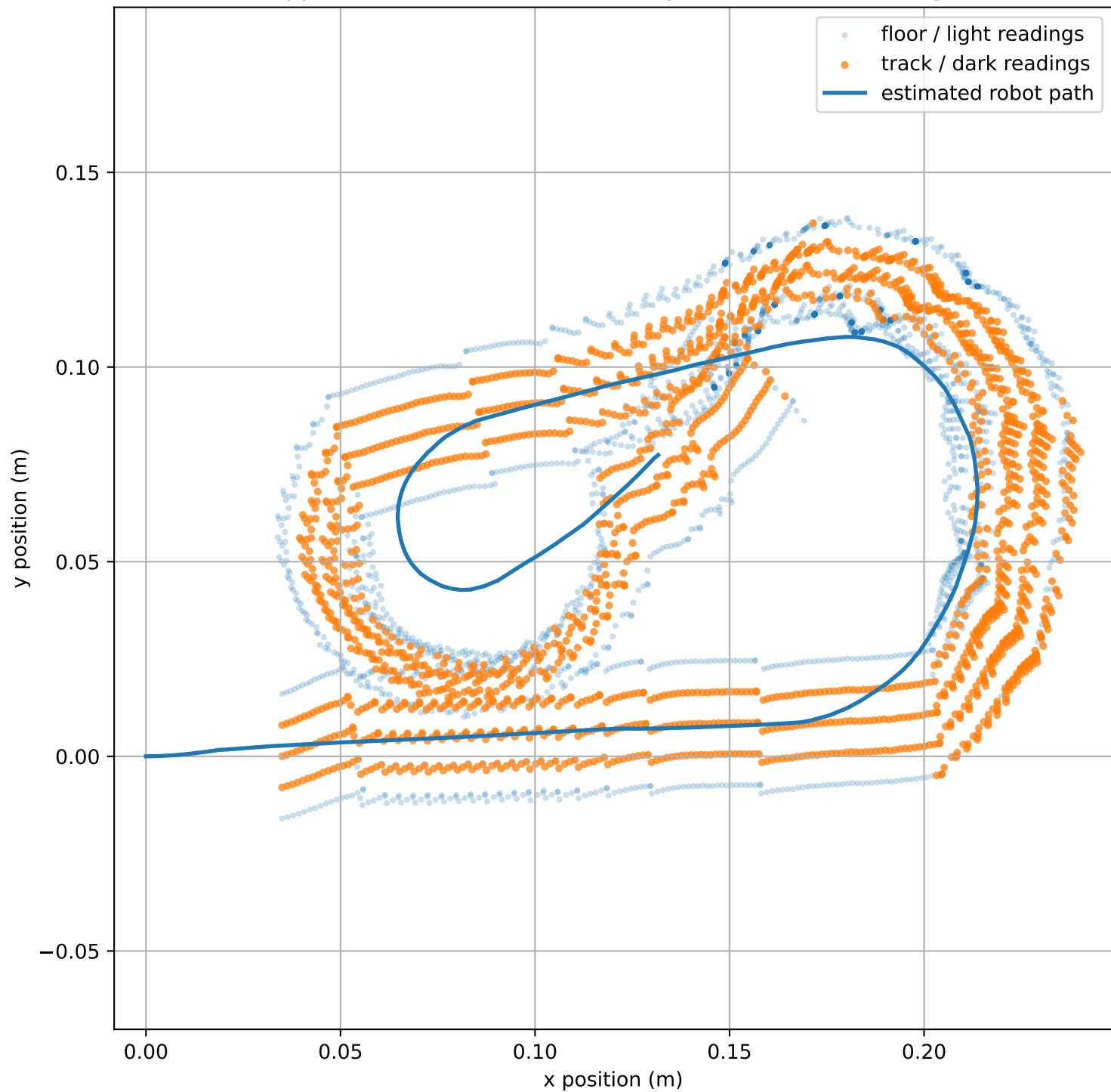
Approximate Pololu 2D Route Map from Line Sensor Logs
