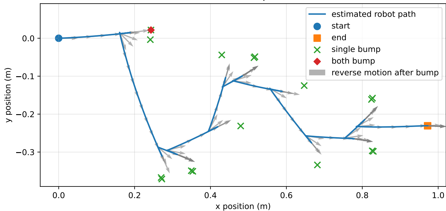
Pololu maze path
