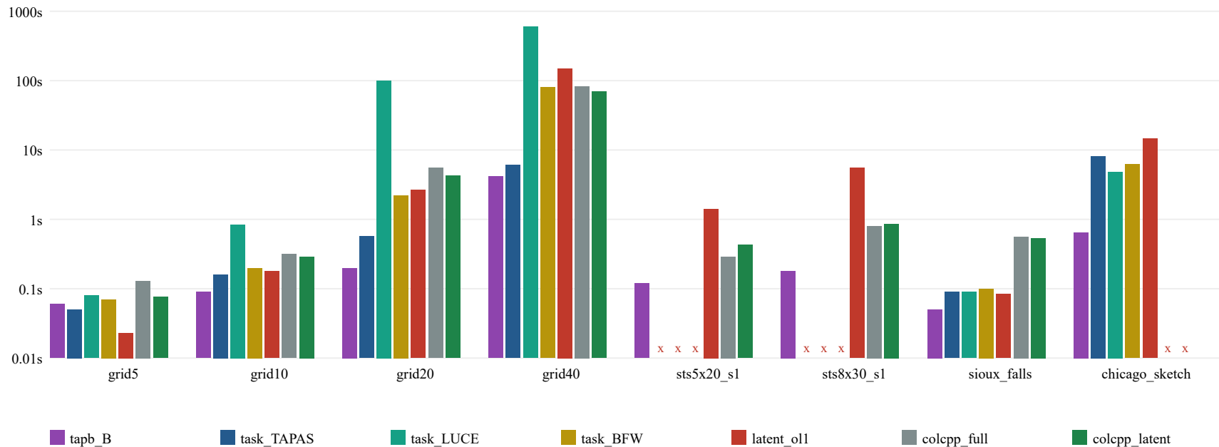
The race: wall time to certified 1e-5 network gap (fixed-pool arms shown at their pool solve)
