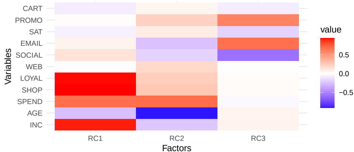
Rotated Loadings Heatmap(varimax)
