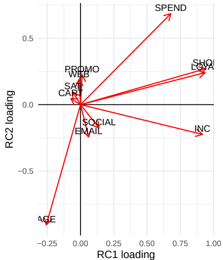
Rotated Loadings Plot (Varimax)
