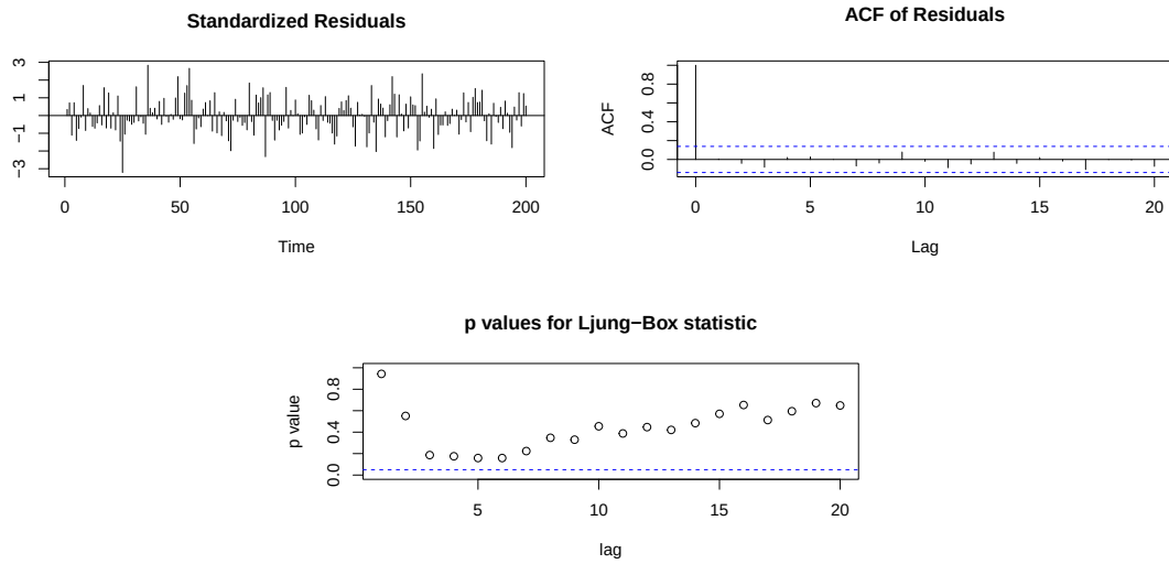
Figure 11: Diagnostic plots for the fitted ARIMA(2,0,2) model for ts2 , including standardized residuals, residual ACF, and Ljung-Box test results.
