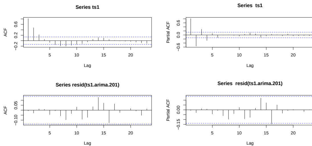
Figure 16: ACF vs PACF of ts1 (top), and of the residuals of fitted ARIMA(2,0,1) (bottom)
