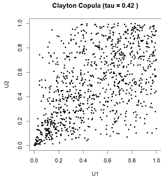
Figure 5: A plot of points generated from Clayton copula. U_1 and U_2 are the quantile of the first and second distribution respectively.
