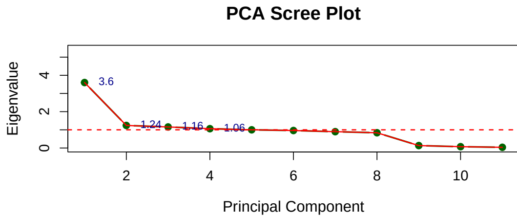
Figure 5: Scree plot
