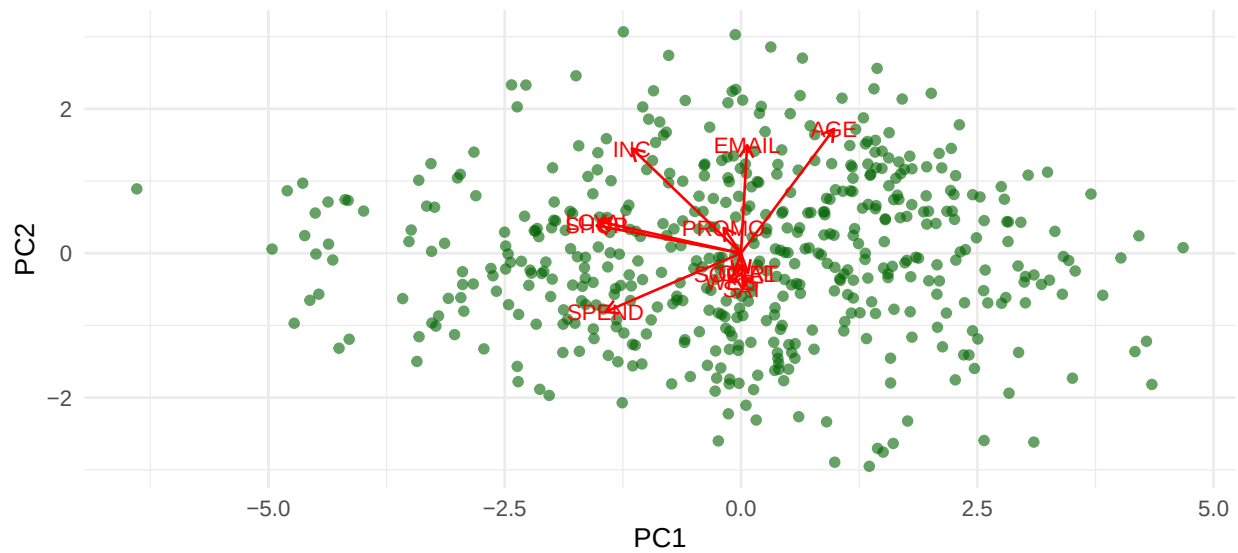
Figure 23: PCA Biplot
