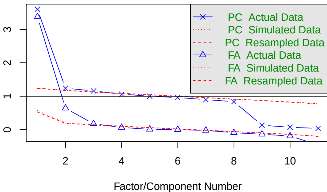
Figure 8: parallel analysis.
