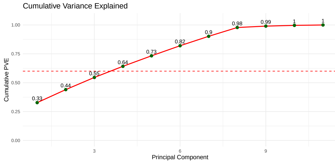
Figure 7: Cumulative variance
