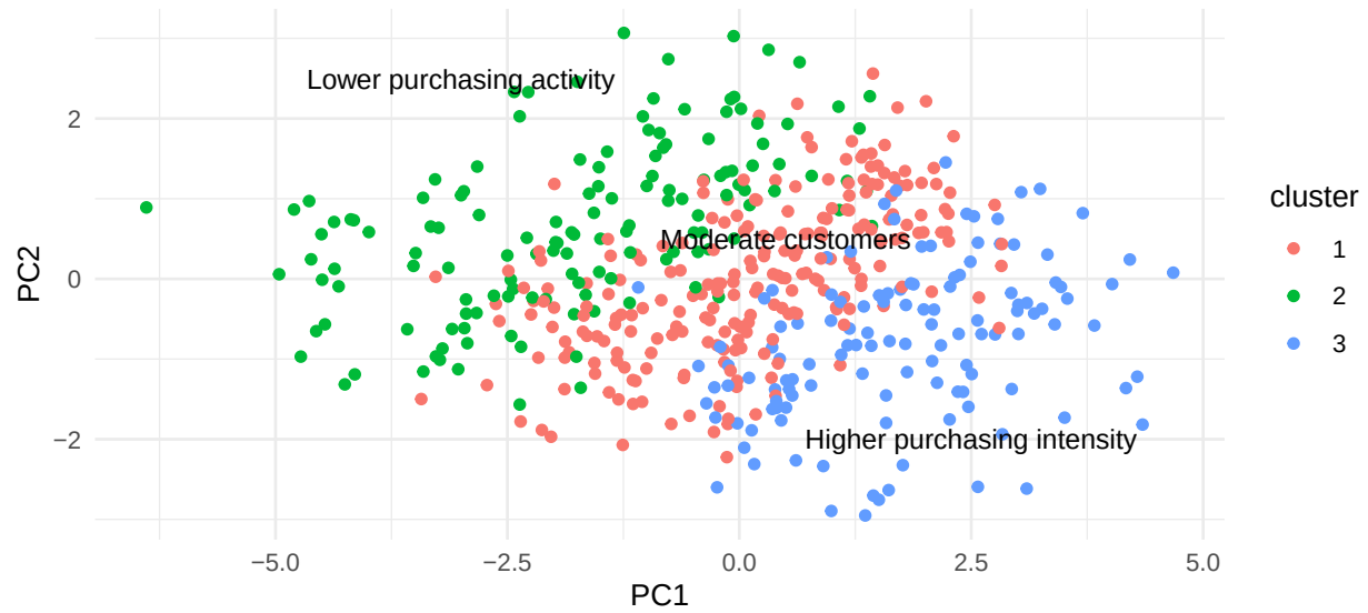
Figure 11: Scatter plot
