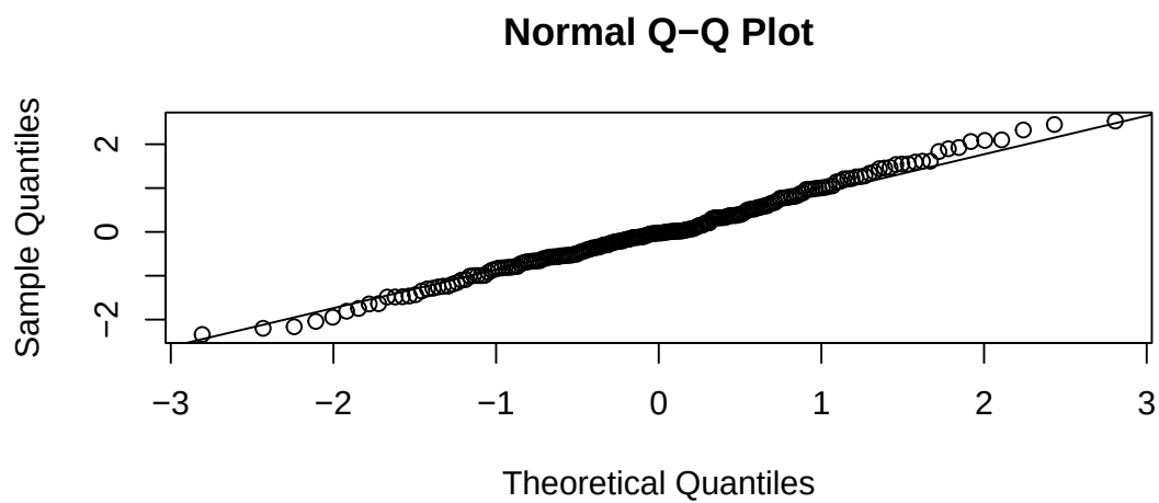
Figure 13: Q-Q plot of the residuals of fitted ARIMA(2,1,0) model for ts3
