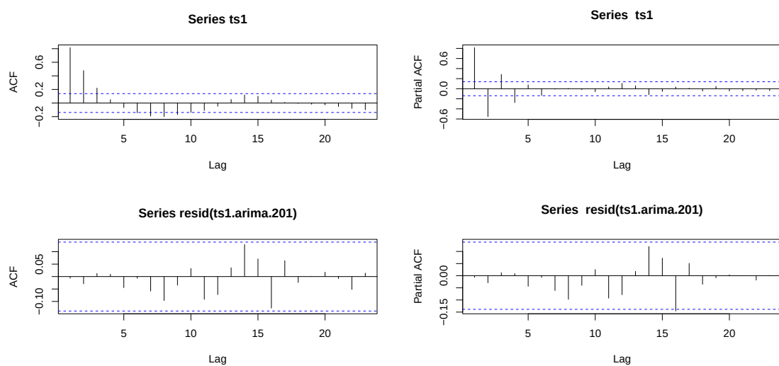
Figure 6: ACF vs PACF of ts1 (top), and of the residuals of fitted ARIMA(2,0,1) (bottom)
