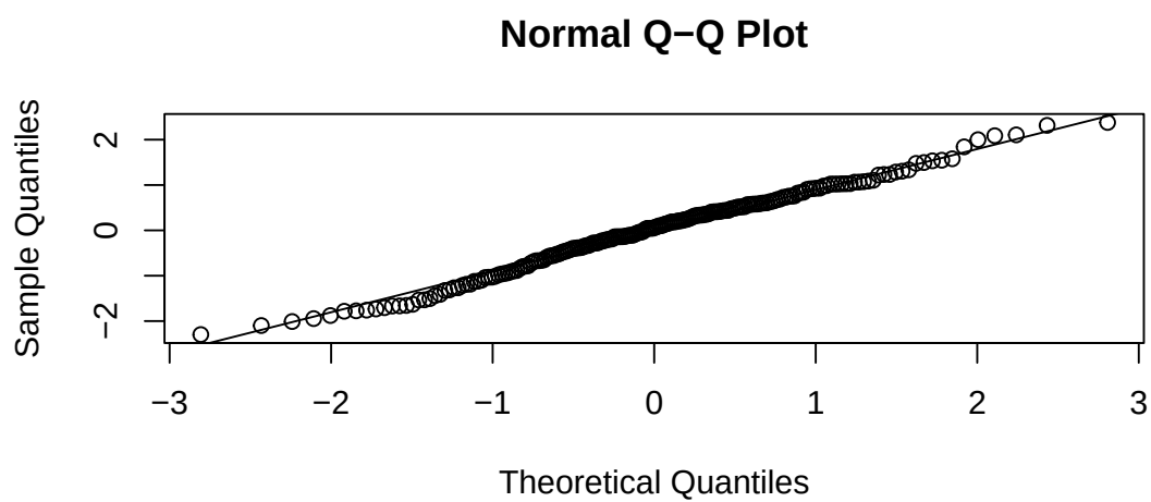
Figure 7: Q-Q plot of the residuals of fitted ARIMA(2,0,1) model for ts1
