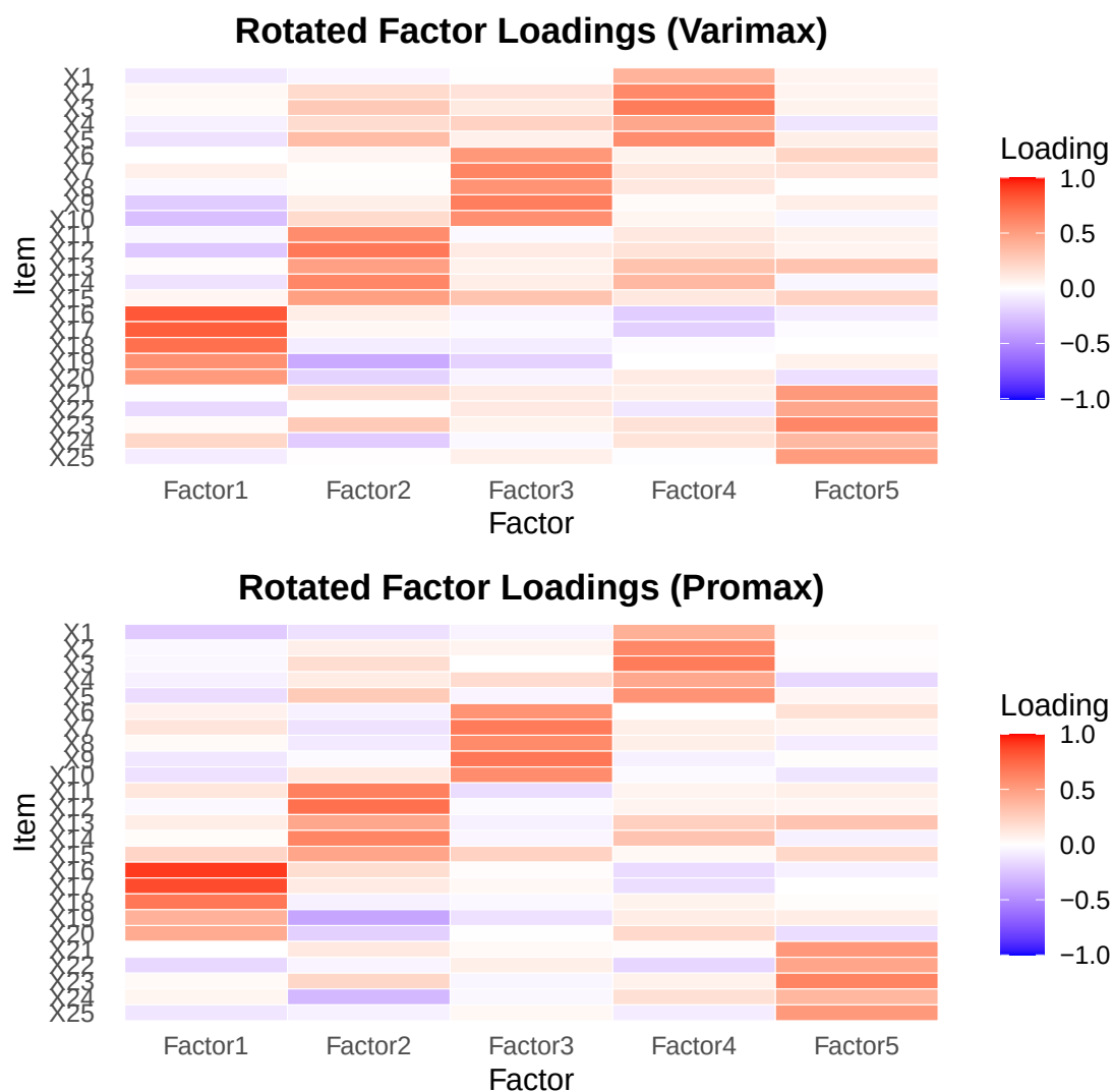
Figure 2: Rotated Factor loadings(Varimax vs Promax)
