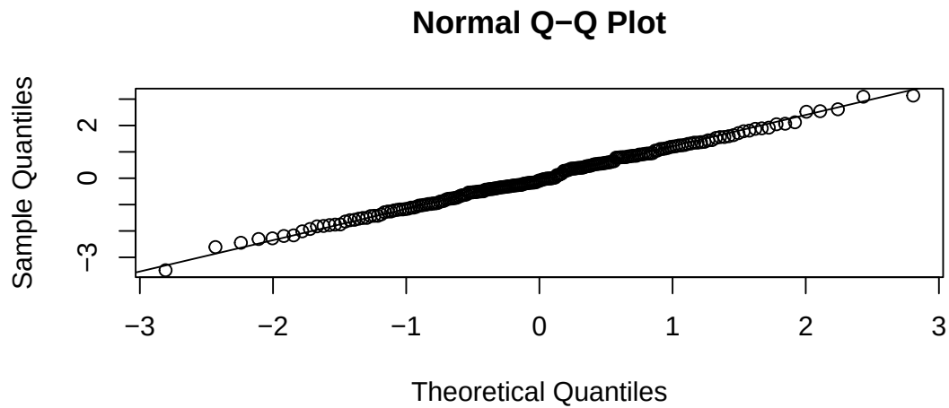
Figure 10: Q-Q plot of the residuals of fitted ARIMA(2,0,2) model for ts2
