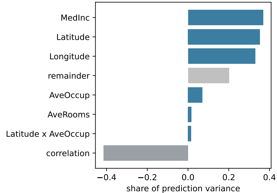
Functional-ANOVA attribution
