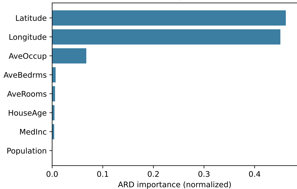
Feature importance
