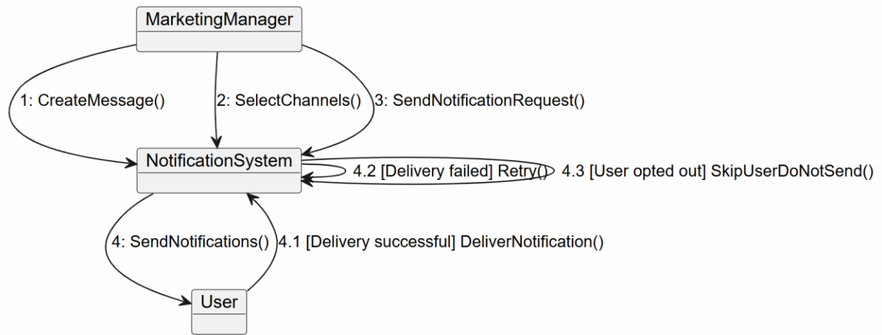
Notification Delivery - Collaboration Diagram
