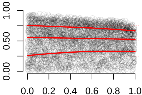
DHARMa residual vs. predicted Quantile deviations detected (red curves) Combined adjusted quantile test significant
