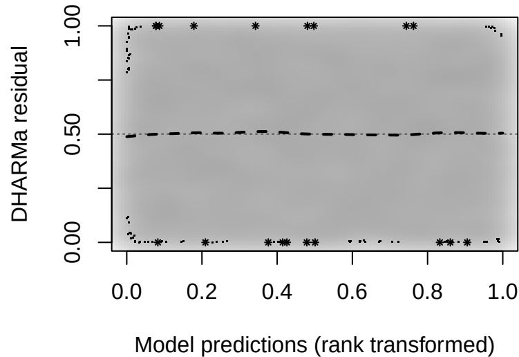
DHARMA residual vs. predicted
