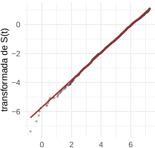
Weibull: \log(-\log S)
