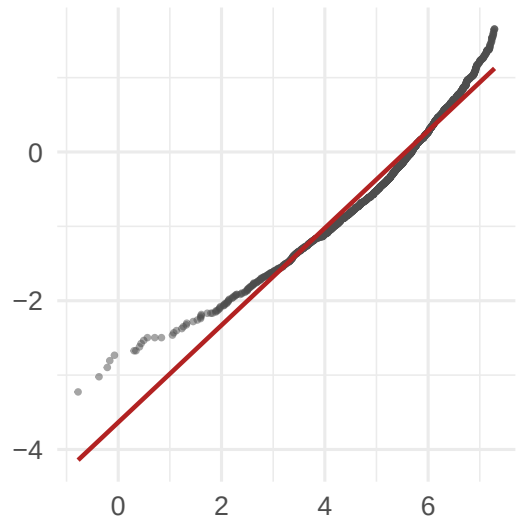
Log-normal: \text{probit}(1-S)
