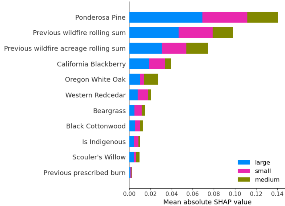
Figure 15: SHAP values for the Random Forest classifier with all plant species counts included separately.
