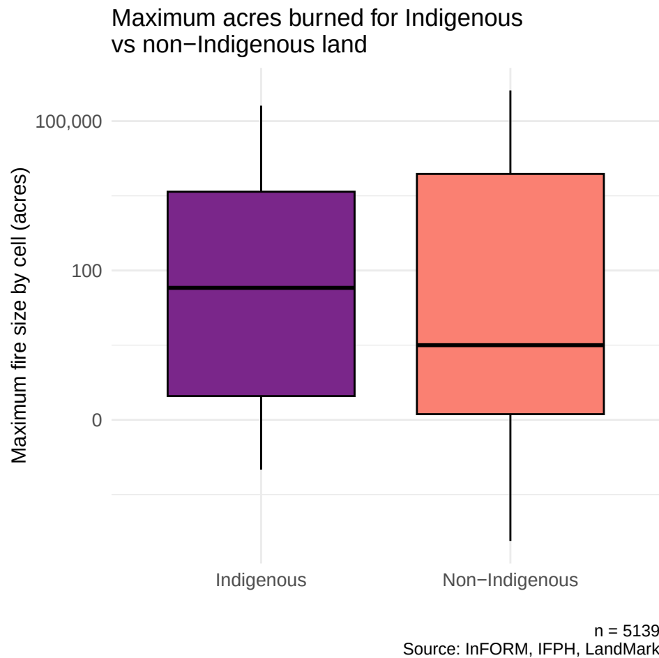
Figure 5: Maximum acres burned across land designation.
