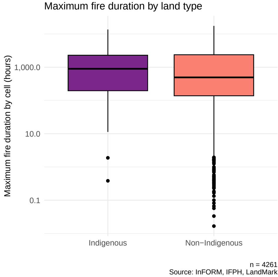
Figure 8: Maximum fire duration across land designation.
