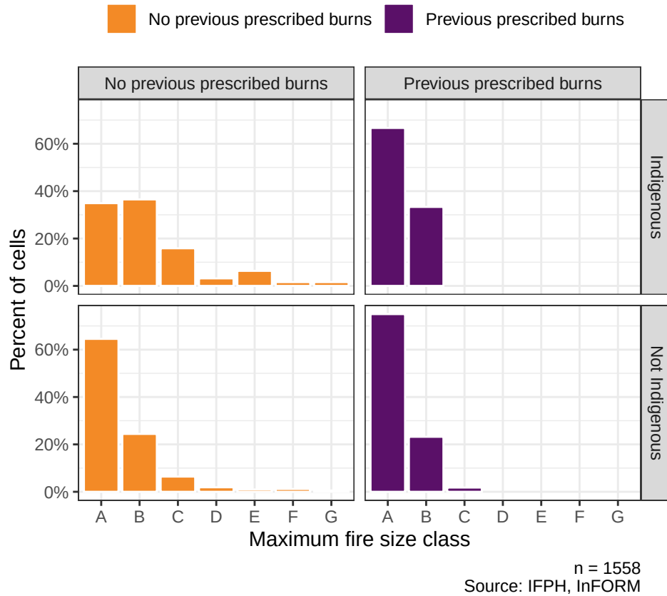
Figure 9: Fire size distribution by prescribed burn history and Indigenous land designation status in 2025.
