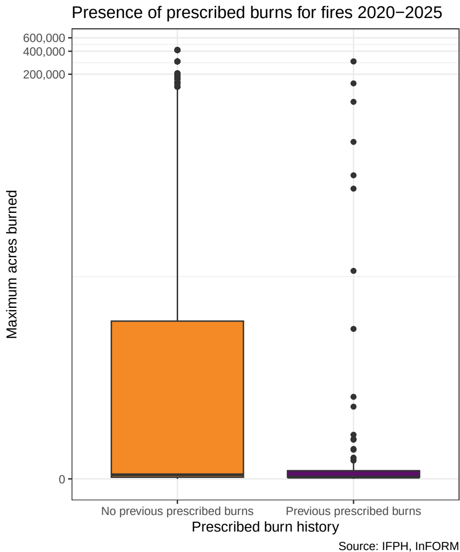
Figure 10: Distribution of fire size between cells that have or have not previously had prescribed burns.
