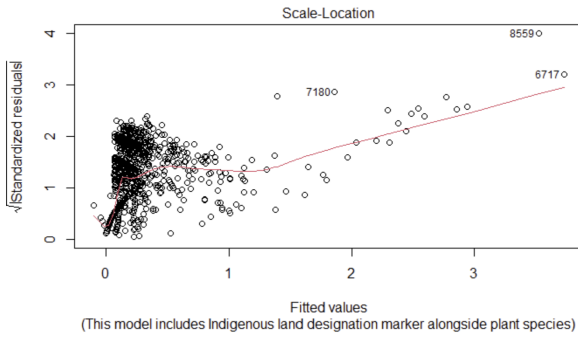
(c) Scale location.
