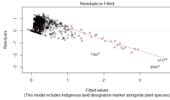
(a) Residuals vs fitted.
