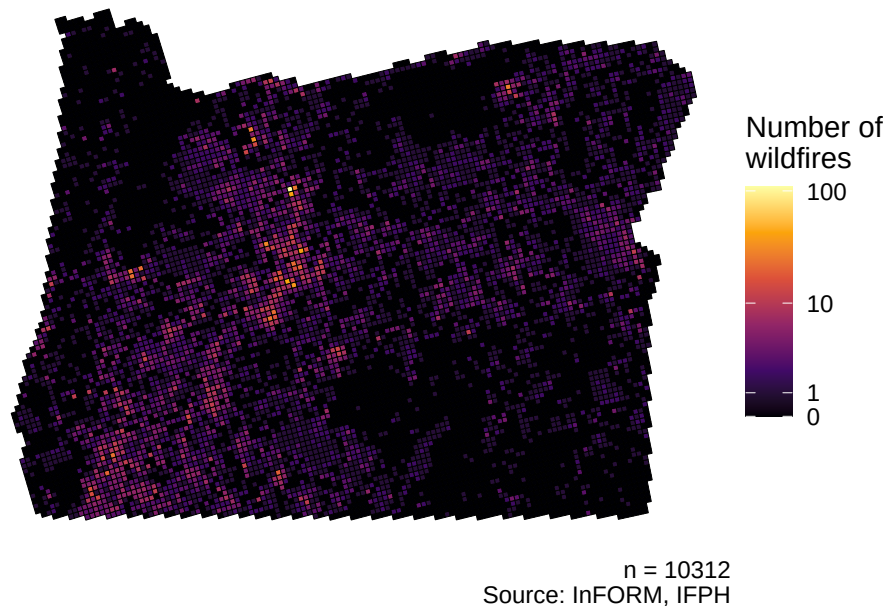
Figure 6: Number of wildfires per cell across Oregon.
