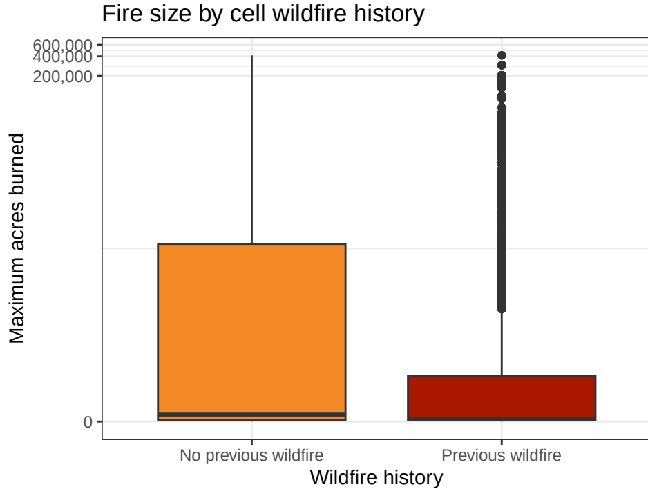
Figure 12: Distribution of fire size between cells that have or have not previously had wildfires.
