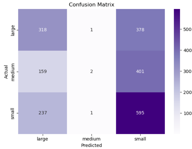
Figure 16: Confusion matrix for the Random Forest classifier.
