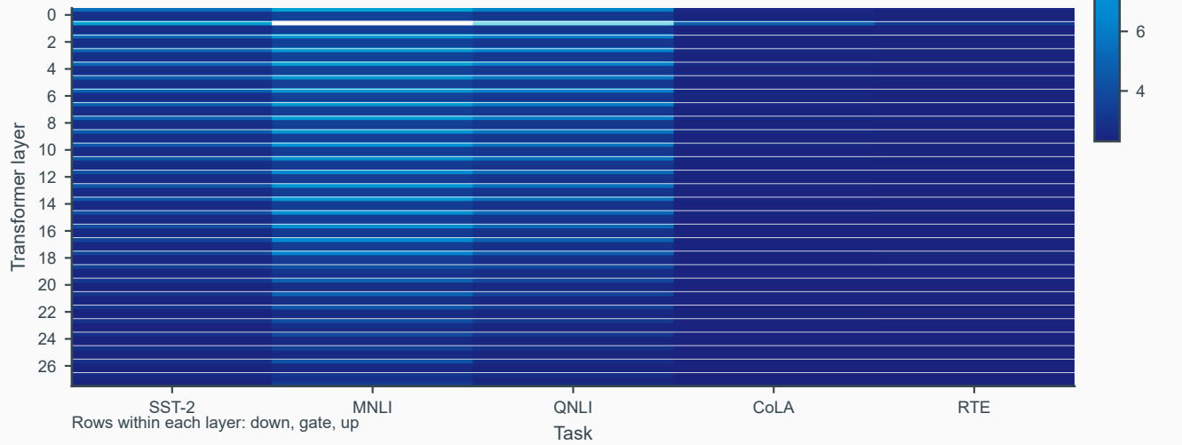
MLP modules: per-layer LoRA A norm
