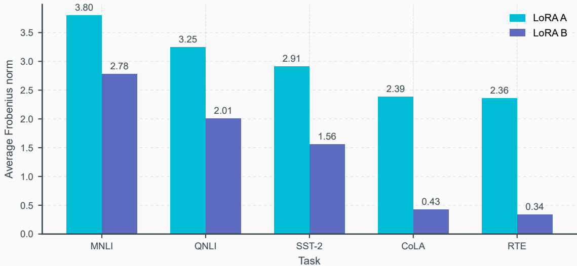
Per-task adapter norm ranking
