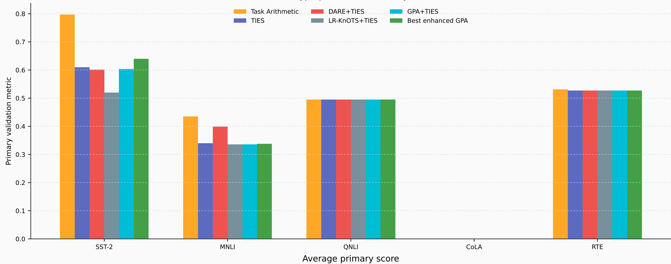
Best hyperparameter results by task
