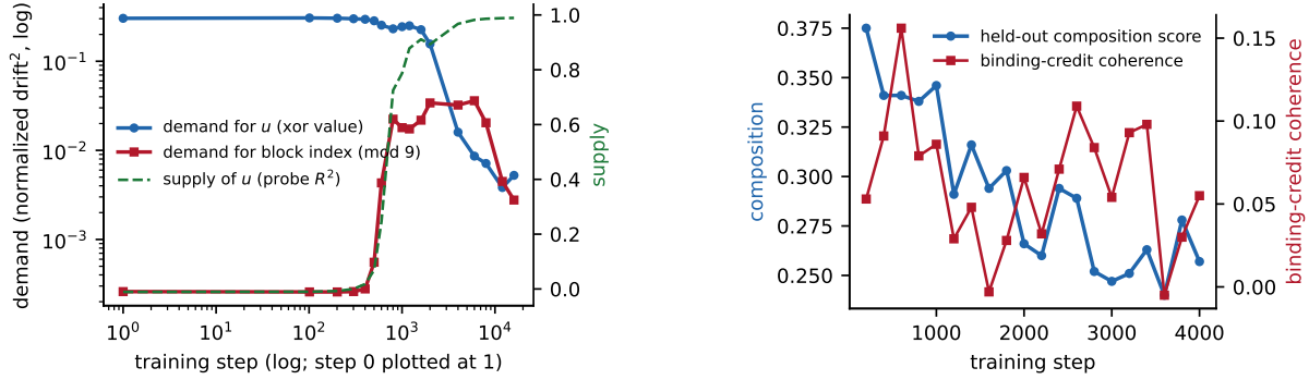
Figure 6: Left: demand and supply at one interface of the matryoshka run. Right: co-financing decoherence in the composition task; held-out composition erodes as the cross-task coherence of the binding-directed credit decays (all 21 checkpoints of the \epsilon = 0.8 run; single seed).
