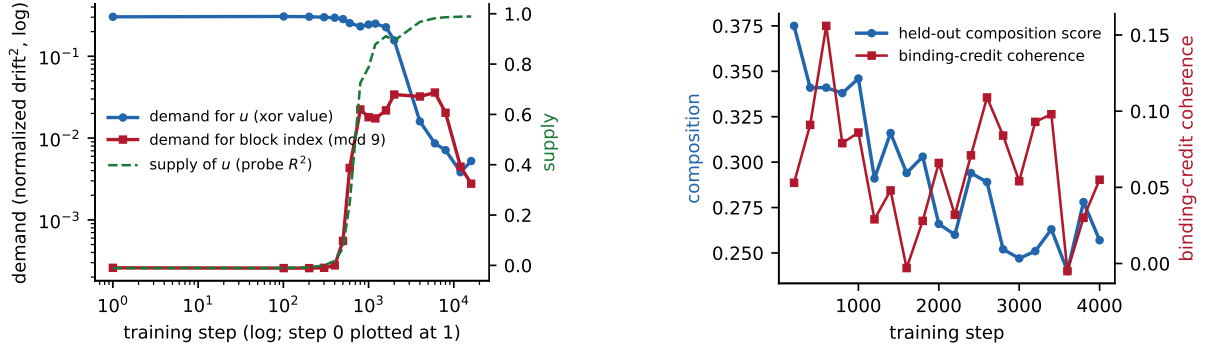
Figure 6: Left: demand and supply at one fixed interface of the matryoshka run (residual stream after block 4; the same measurement at other depths is summarized in the text). Right: co-financing decoherence in the composition task; held-out composition erodes as the cross-task coherence of the binding-directed credit decays (all 21 checkpoints of the \epsilon = 0.8 run; single seed).
