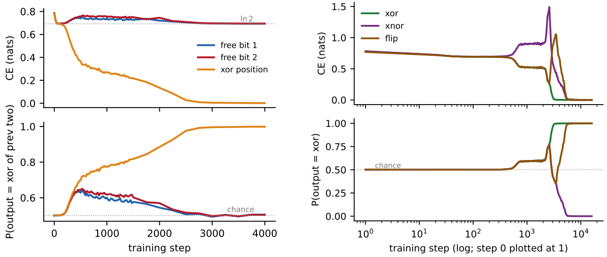
Figure 5: Left: RRXOR formation; per-class CE (top) and probability of outputting the xor of the previous two bits (bottom); the two free-bit classes nearly coincide throughout, as symmetry demands. Right: the matryoshka cascade (period-27 exception tower over the xor rule: XNOR at two of nine blocks, one block flipping back); the exception classes’ CE spikes exactly while the model’s probability of outputting plain xor on them rises : the net confidently bets the wrong rule until the correction that distinguishes the blocks is financed by those very errors.
