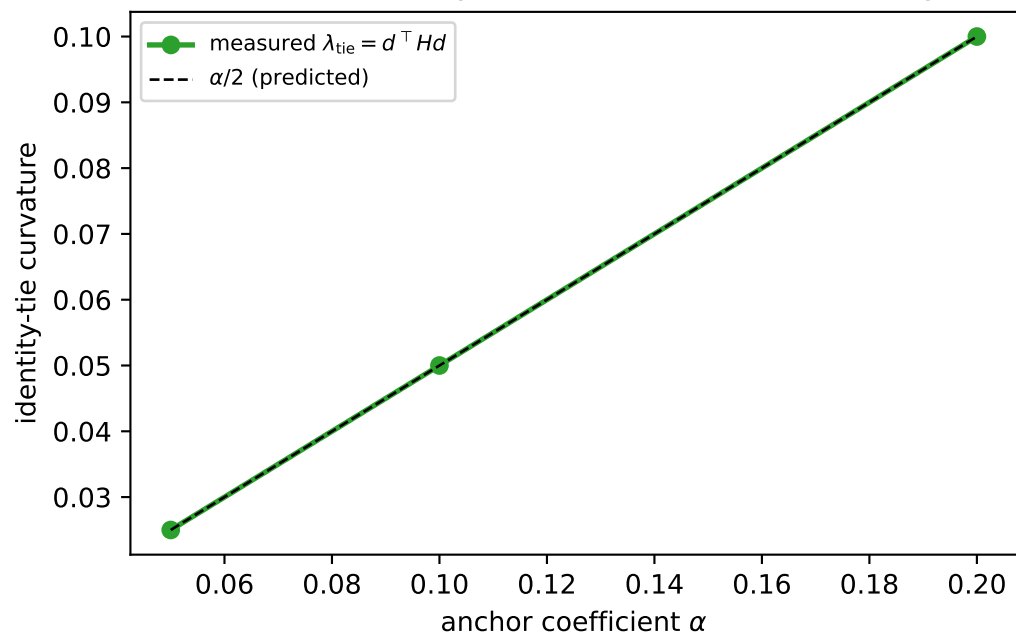
(d) without redundancy, the anchor restores identity at \alpha/2
