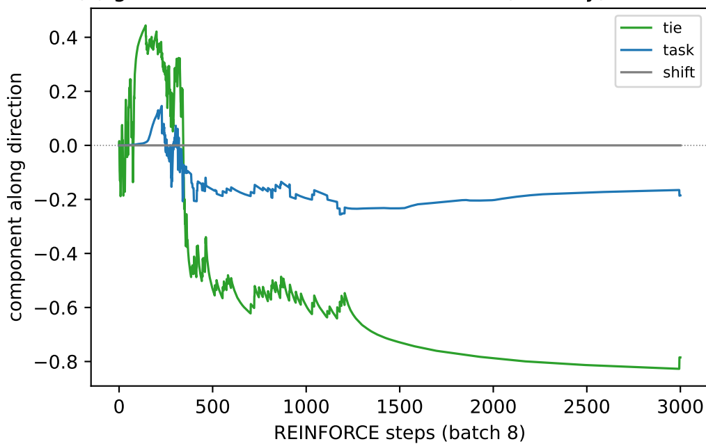
(c) gradient noise lives on the interior (identity) directions
