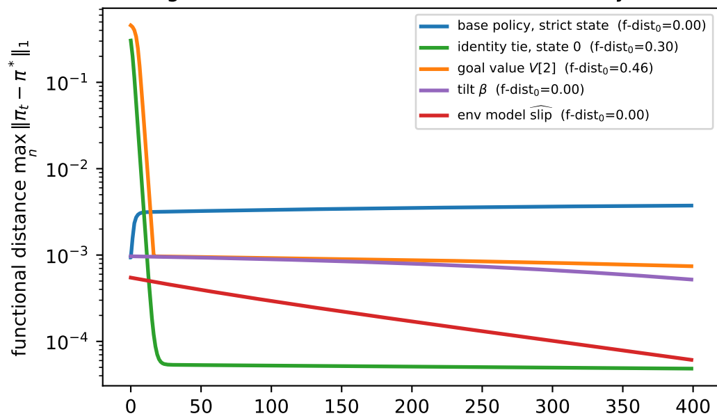
(a) gradient flow heals the function, block by block
