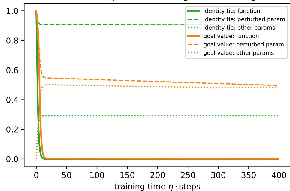
(d) without redundancy, the anchor restores identity at \alpha/2
