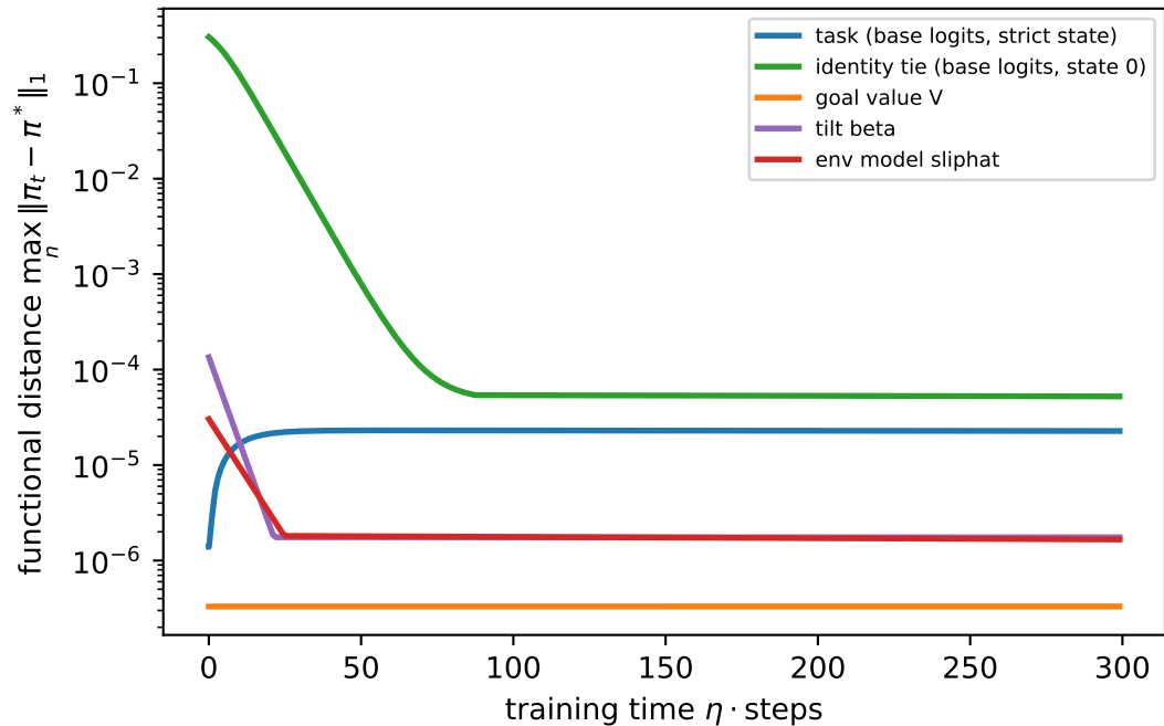
gradient flow heals the FUNCTION (rates differ by block)
