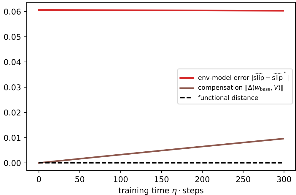
the weight-space scar: function heals, parameters migrate
