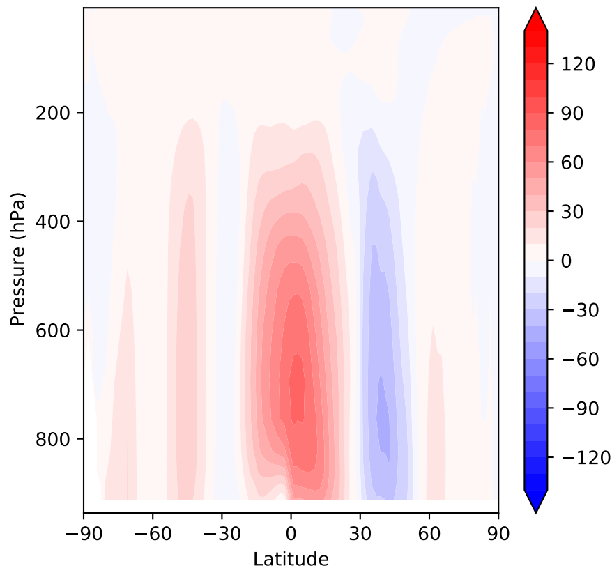
Meridional streamfunction, 0 (Sv)
