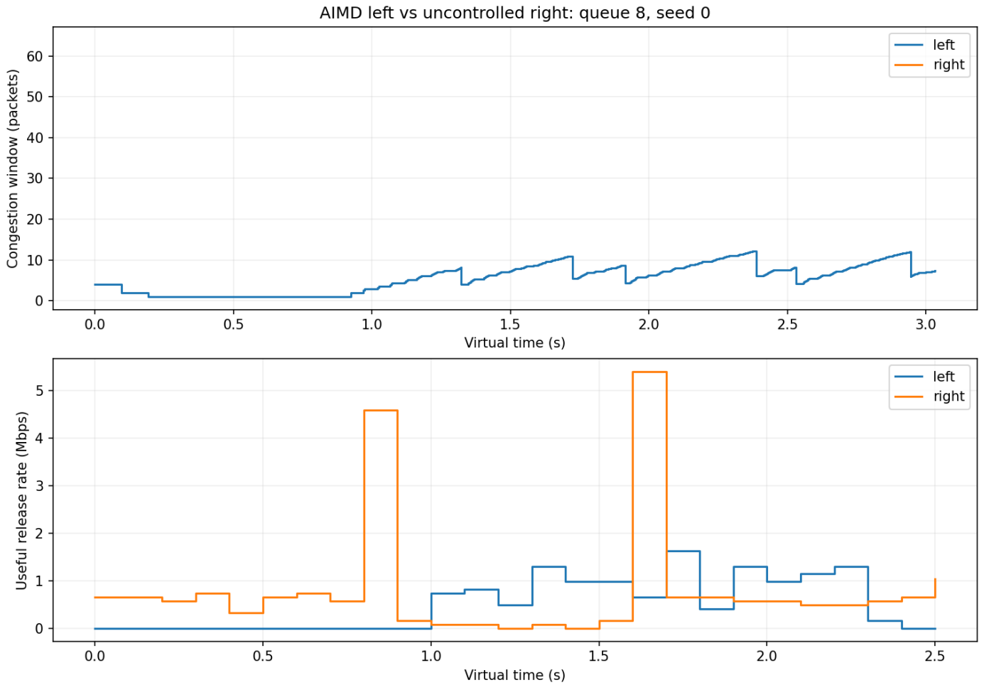
Congestion window and useful release rate: AIMD versus uncontrolled
