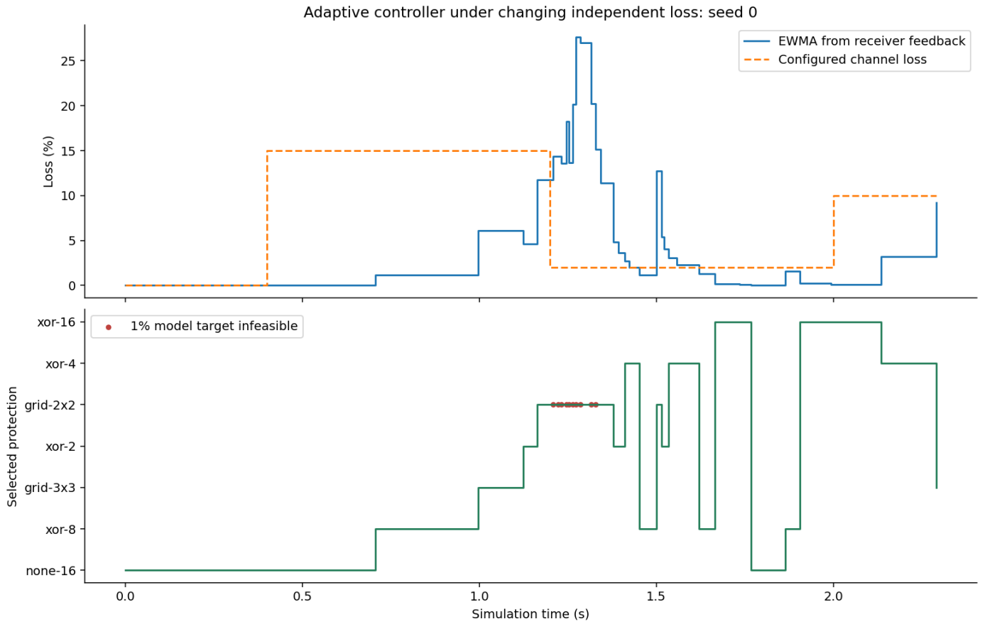
Applied adaptive controller decisions in changing loss
