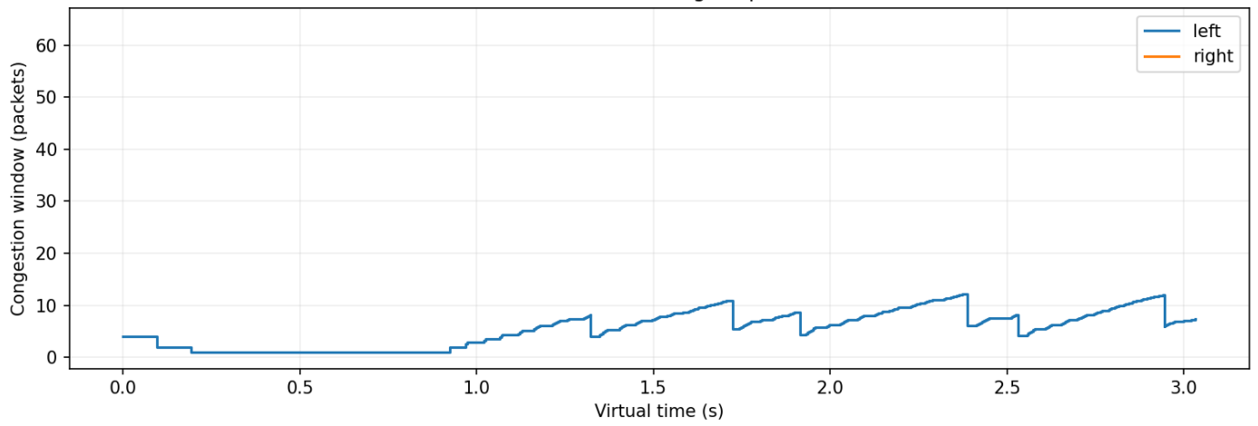
AIMD left vs uncontrolled right: queue 8, seed 0
