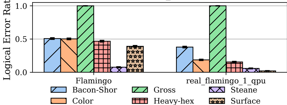
DQC IBM Flamingo (error_rate=10) Lower is better ↓
