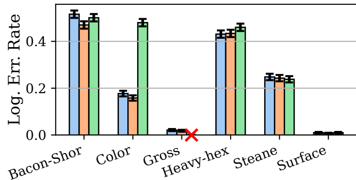
a) Effectiveness Lower is better ↓
