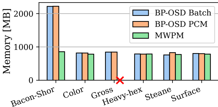
c) Memory Lower is better ↓
