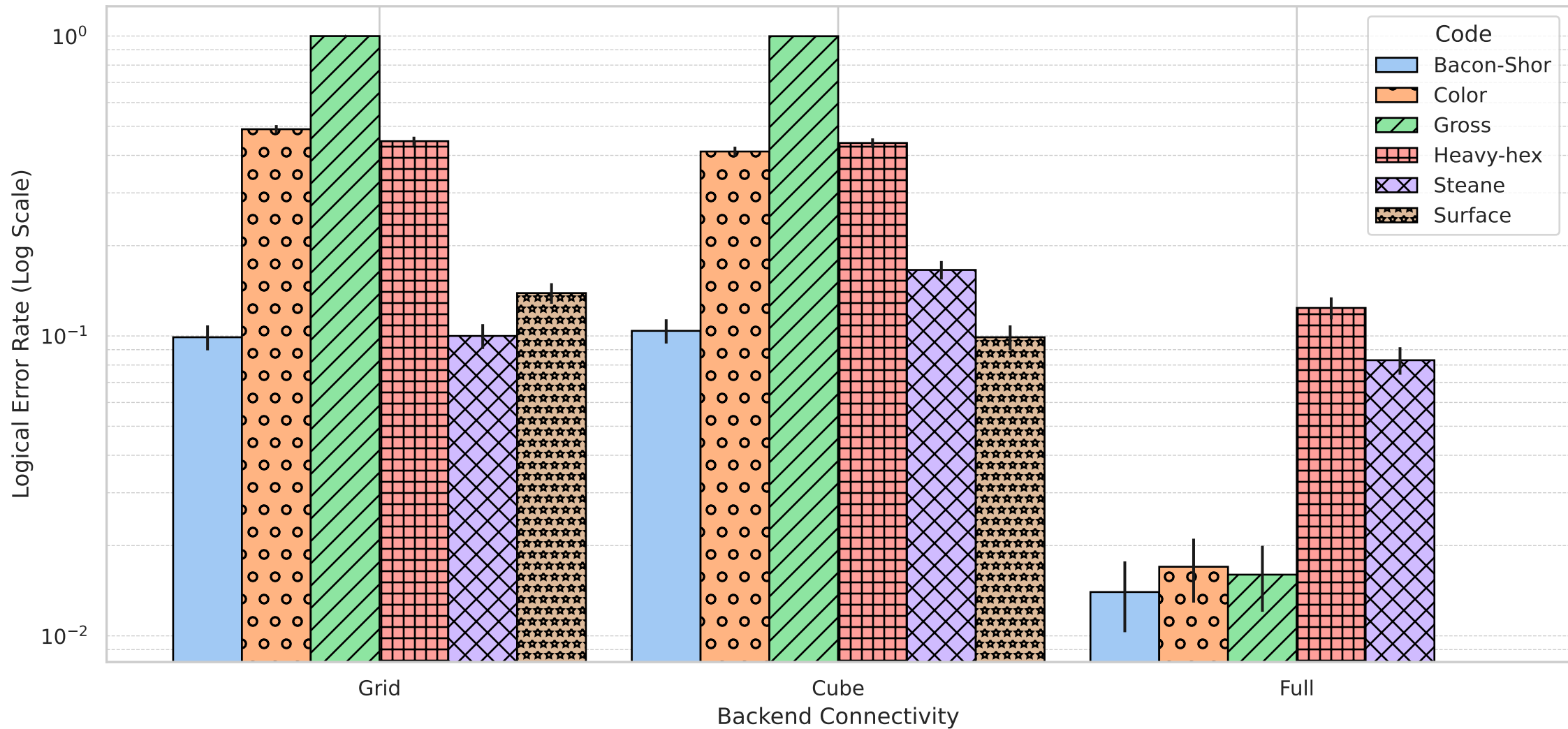
Logical Error Rate by Backend
