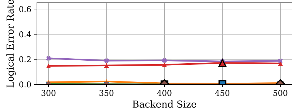
(a) Constant ( p=0.002 ) Lower is better ↓
