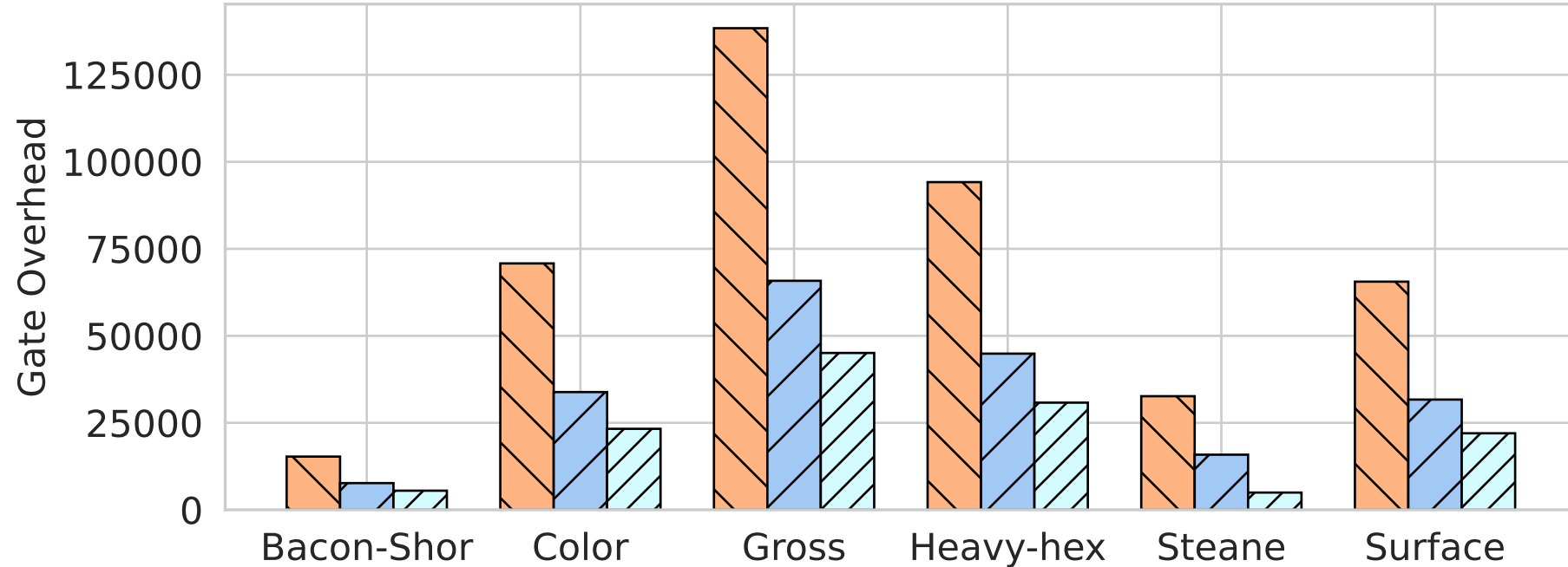
(a) Gate Overhead (IBM Heron)
