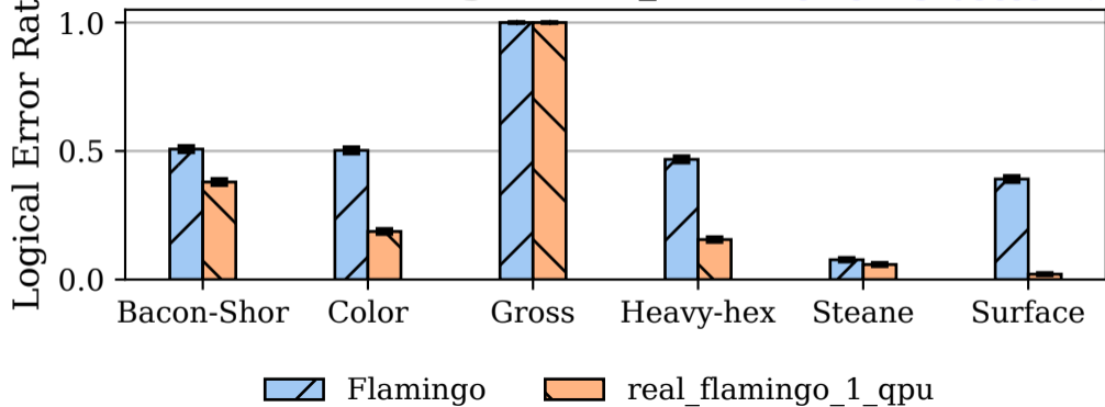
DQC IBM Flamingo (error_rate=1) Lower is better ↓
