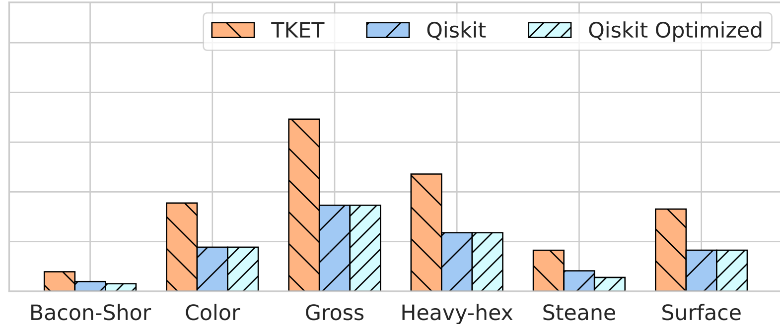
(b) Gate Overhead (H2)
