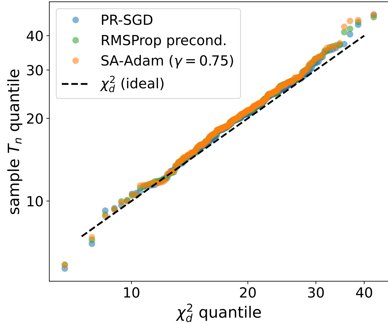
(a) Adaptivity is invisible ( n = 10^8 , d = 20 )
