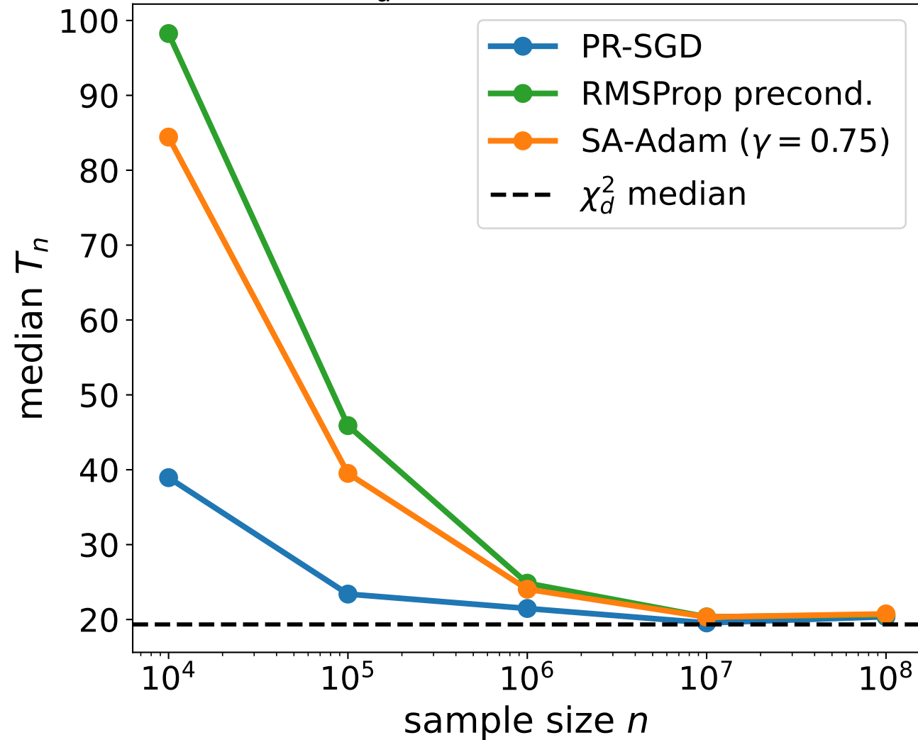
(b) median T_n \rightarrow \chi_d^2 median (adaptivity washes out)
