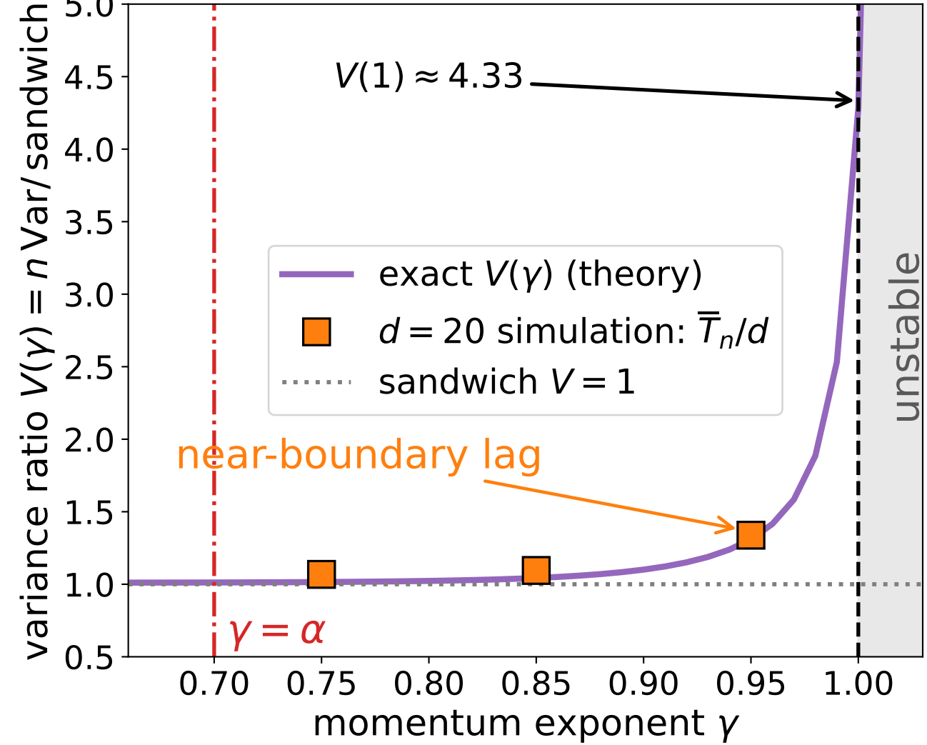
(c) Necessity of \gamma < 1 : formula is exact
