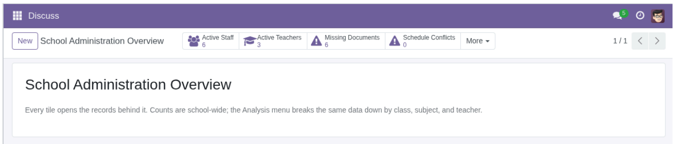
Figure 1 — Administrator overview, section 10. Counts are read live from the database and each tile opens the records behind it. Schedule conflicts read zero because the create and write constraints reject clashes at source. This screen previously rendered every tile as zero; that was defect 11. The sixth staff record was added during manual testing after the demo data shipped with five.
