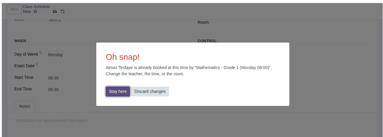
Figure 2 — Conflict validation, section 7.3. An attempt to schedule Almaz Tesfaye for Grade 2 A on Monday from 08:30 to 09:30 is rejected because she already teaches Grade 1 A from 08:00 to 09:00. The message names the clashing record. This is a backend constraint raised on create, not a user-interface warning, which section 7.3 states explicitly is not sufficient on its own.
