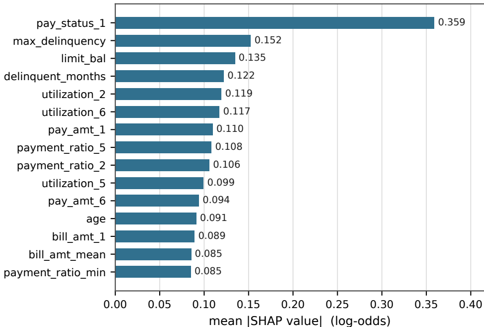
Global feature attribution, lightgbm (TreeExplainer(exact)) top 15 of 49 predictors, 300 evaluation rows
