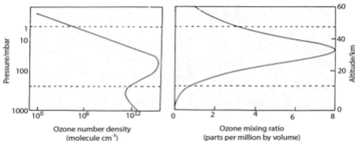
Figure 1.6 — Variation of ozone concentration with altitude, expressed as an absolute number density ( n_{O_3} , with peak just above 10^{12} \text{ cm}^{-3} ) and as a mixing ratio (mole fraction, n_{O_3}/n_{air} ).
