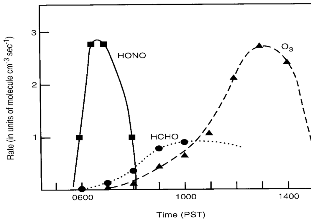
Figure 7.3 — Overview of different sources of HOx during the day .
