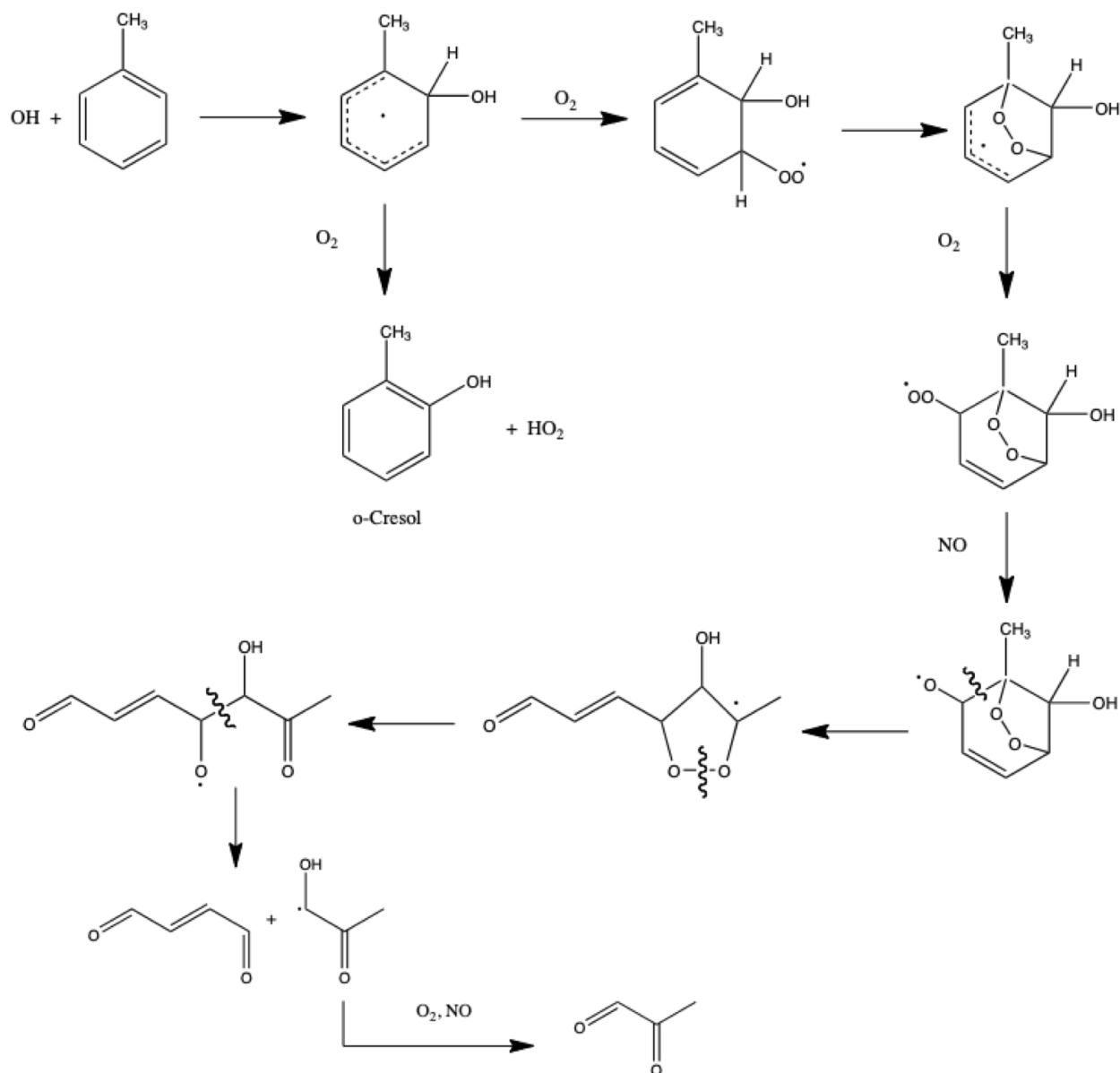
Figure 11.3 — OH initiated oxidation mechanism of toluene
