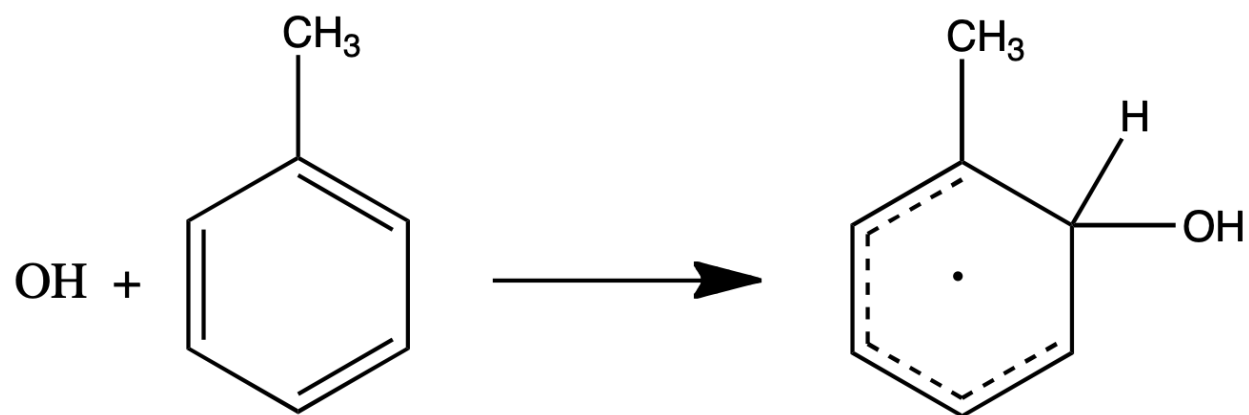
Figure 11.2 — OH addition in the oxidation of Benzene
