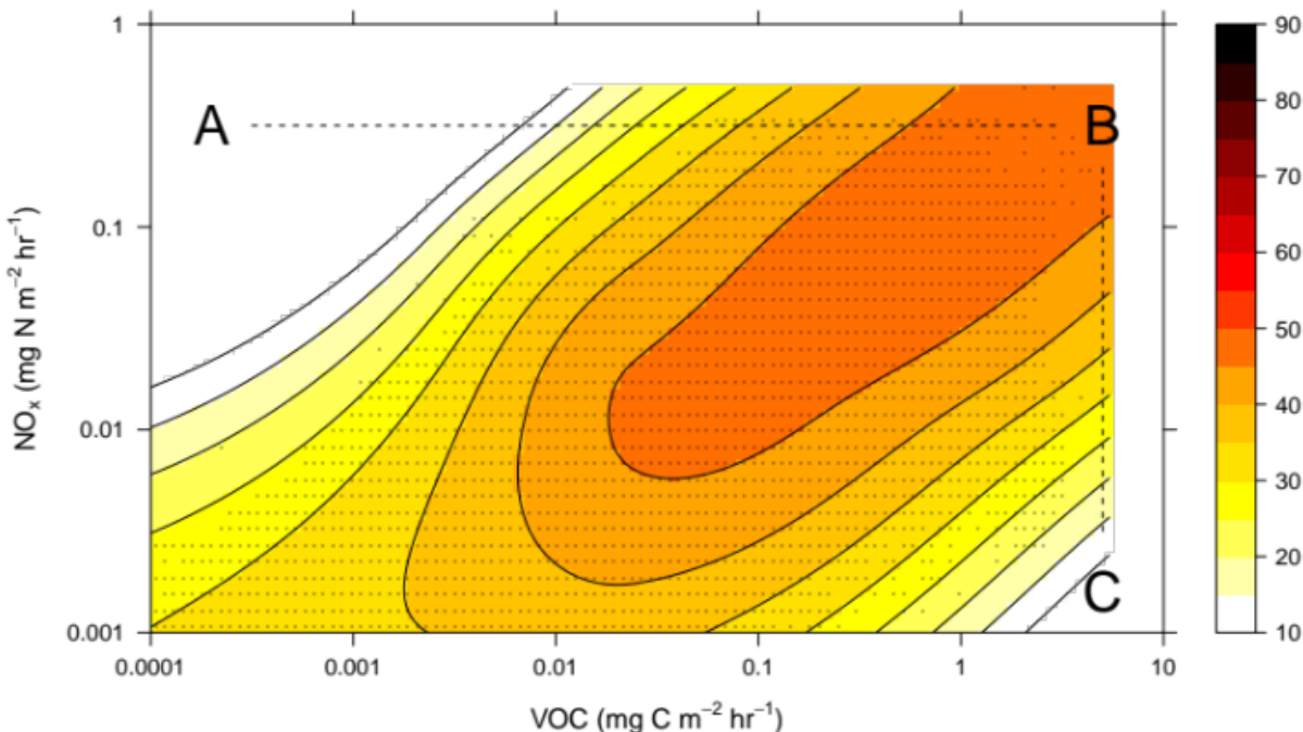
Figure 8.6 — Modelled ozone mixing ratio (ppb) as a function of NO x emission rate and VOC emission rate.
