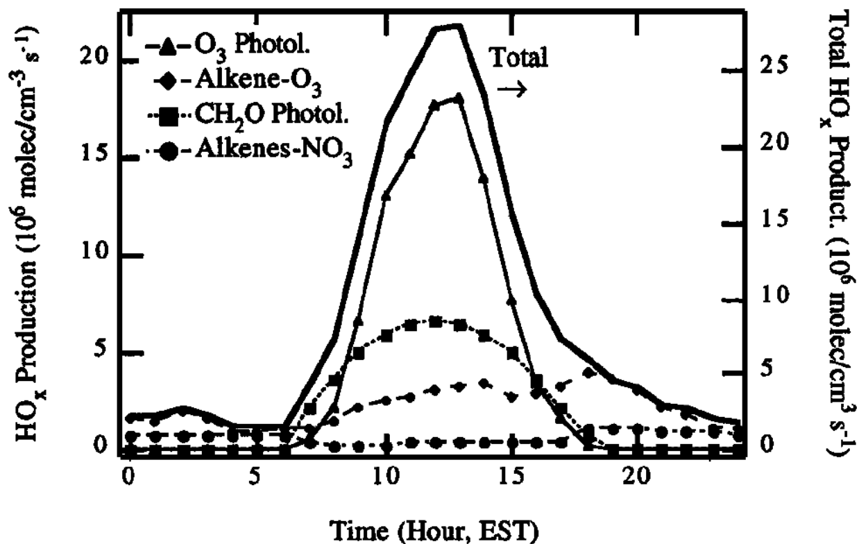
Figure 10.7 — Calculated rates of HO x generation from various sources at a rural site (Paulson and Orlando,
