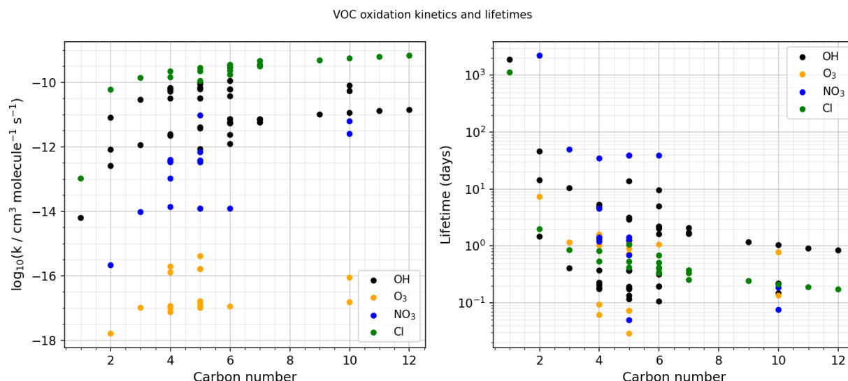
Figure 10.1 — Reaction rate constants for VOCs with different carbon number with different oxidants; corresponding lifetimes to oxidation given [\text{OH}] = 1 \times 10^6 \text{ cm}^{-3} ; [\text{Cl}] = 1 \times 10^5 \text{ cm}^{-3} ; [\text{NO}_3] = 1 \text{ ppt} and [\text{O}_3] = 40 \text{ ppb} .
