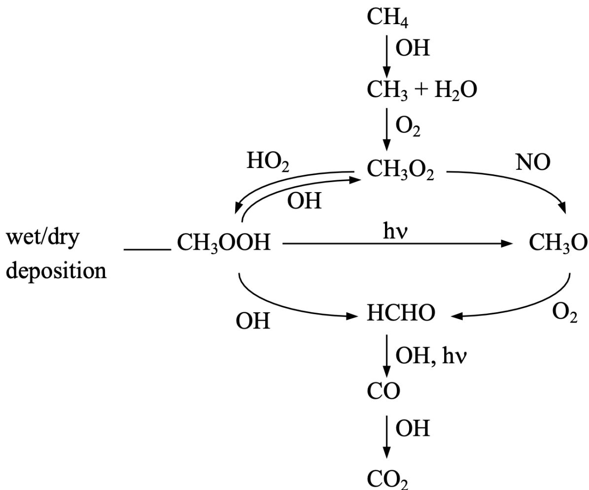
Figure 8.1 — Atmospheric oxidation scheme for methane.
