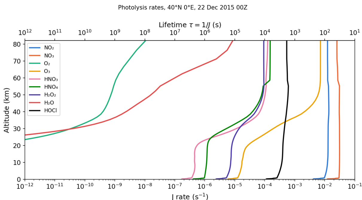
Figure 3.14 — Overview of the photolysis coefficients of important trace gases in the stratosphere.
