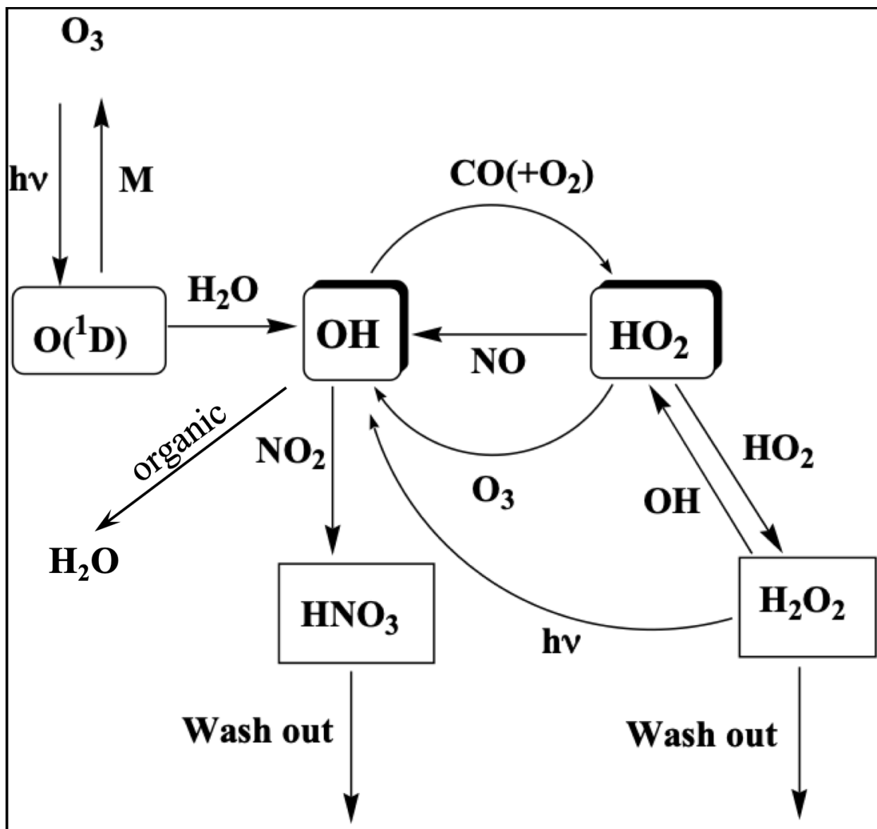
Figure 7.4 — Schematic of reactions governing HOx radicals in troposphere.
