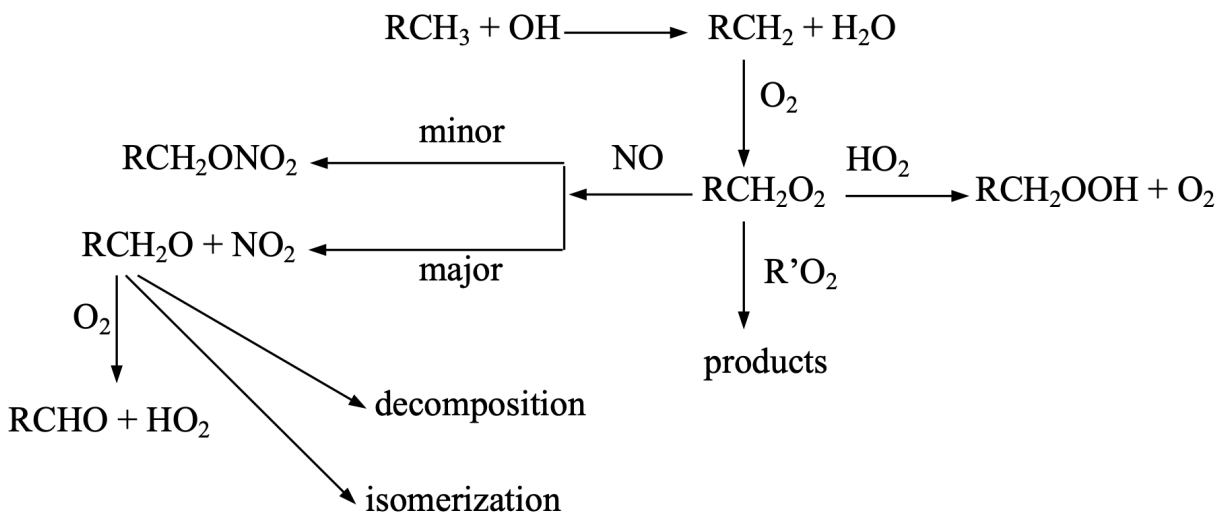
Figure 10.2 — OH initiated oxidation mechanism of alkanes.
