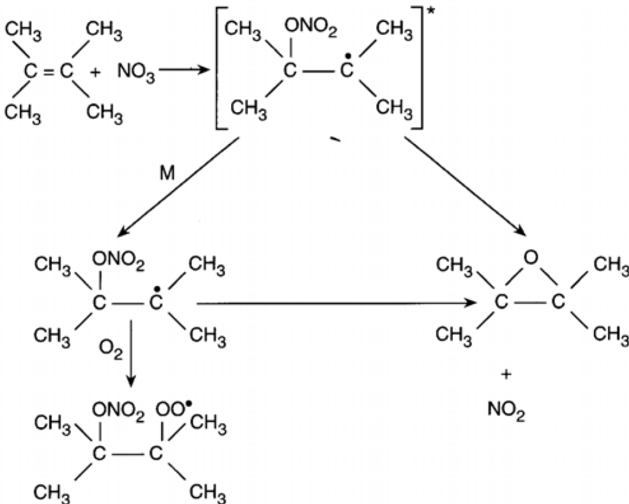
Figure 10.3 — NO_3 oxidation of alkenes proceeds via addition to the double bond. At low pressures (not common in the atmosphere) an epoxide may form.
