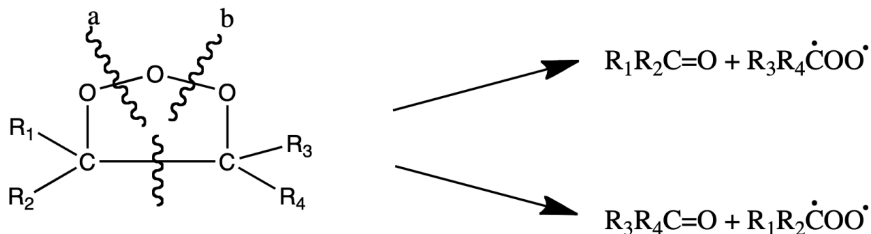
Figure 10.4 — Generation of Criegee intermediate/carbonyl oxide from alkene ozonide reaction.
