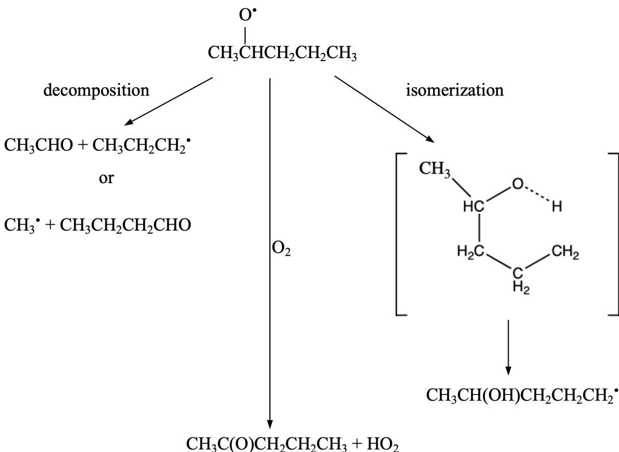
Figure 10.2 — Decomposition of alkoxy radicals under tropospheric conditions.
