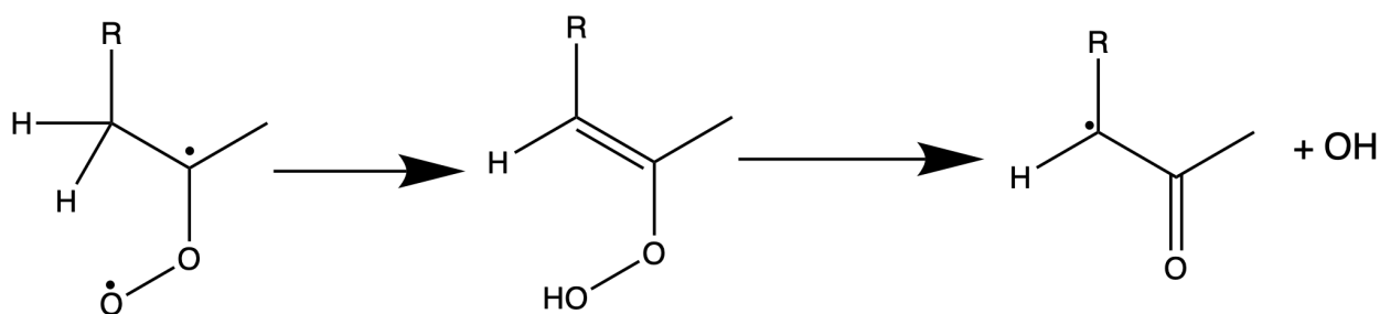
Figure 10.5 — OH generation from “hot” Criegee intermediate
