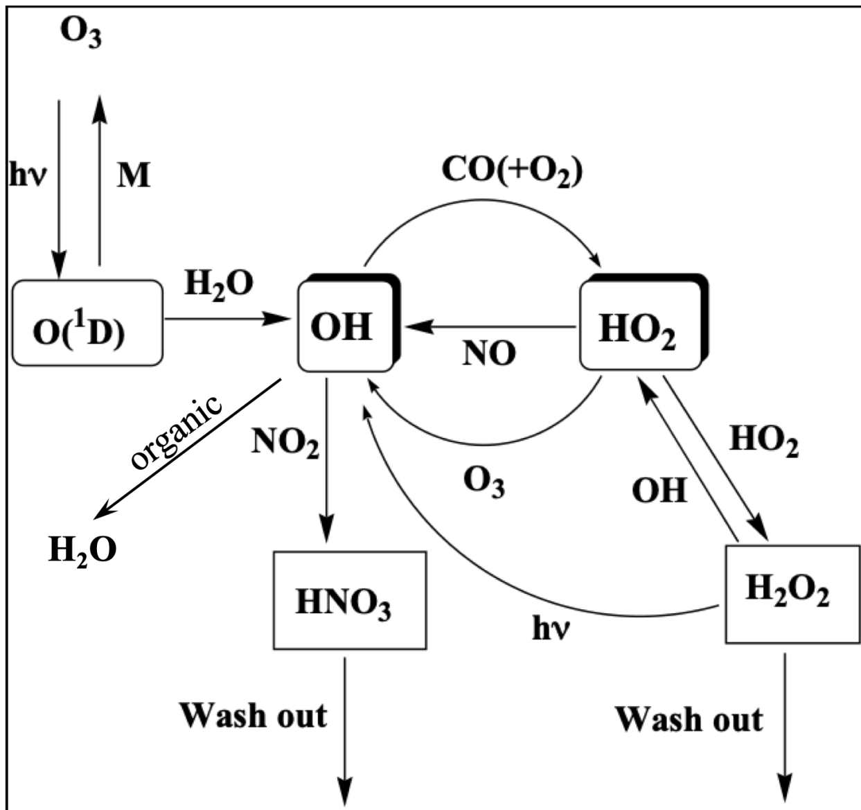
Figure 7.3 — Schematic of reactions governing HOx radicals in troposphere.
