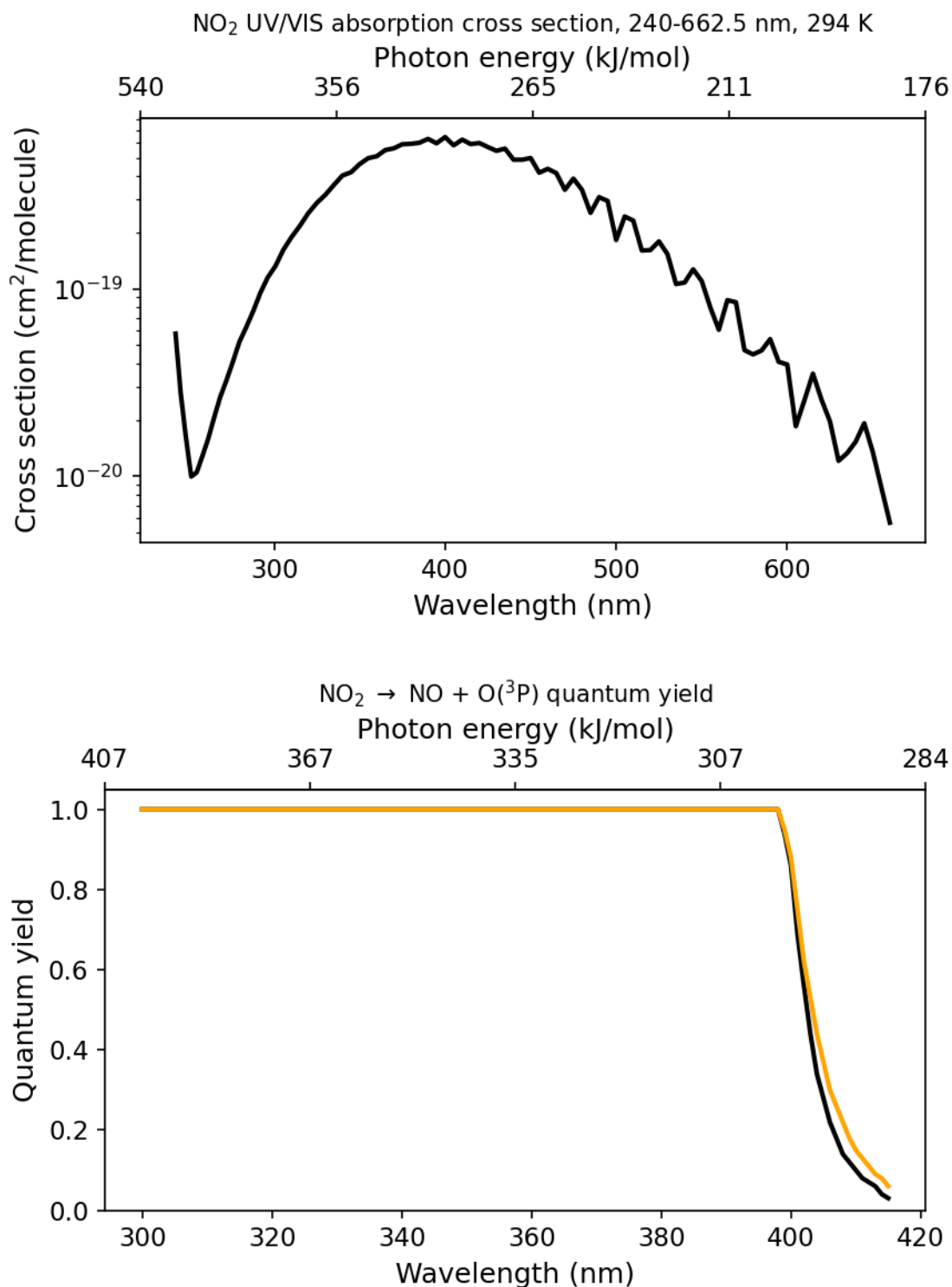
Figure 3.9 — NO 2 absorption cross-section and quantum yield.
