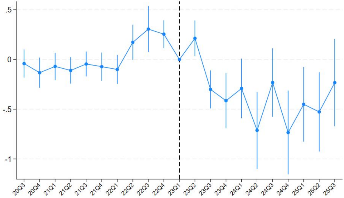
Figure 1: Event Study: Introduction of ChatGPT-4
