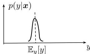
Figure 13: Somewhat easy posterior
