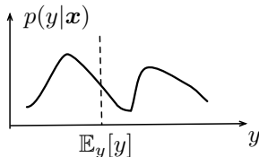
Figure 12: Somewhat difficult posterior
